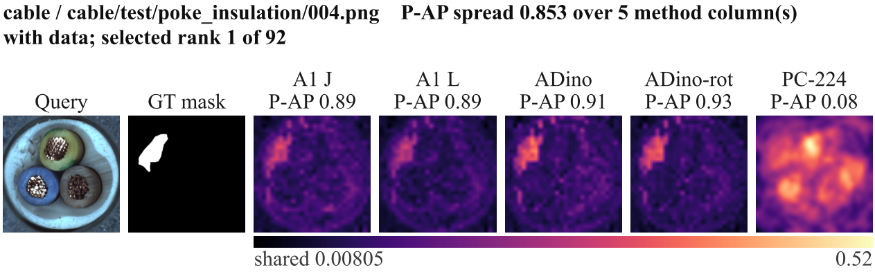
Figure 7 - mvtec cable: multi-method per-sample comparison on the S8 common region (seed 0, K 4; region 392 x 392, 76.6% of the canvas)
