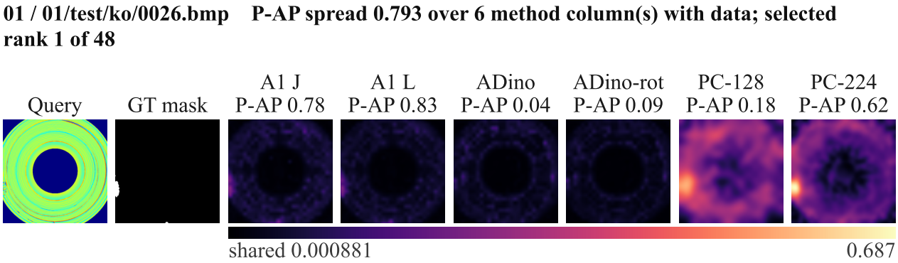
Figure 7 - btad 01: multi-method per-sample comparison on the S8 common region (seed 0, K 4; region 392 x 392, 76.6% of the canvas)
