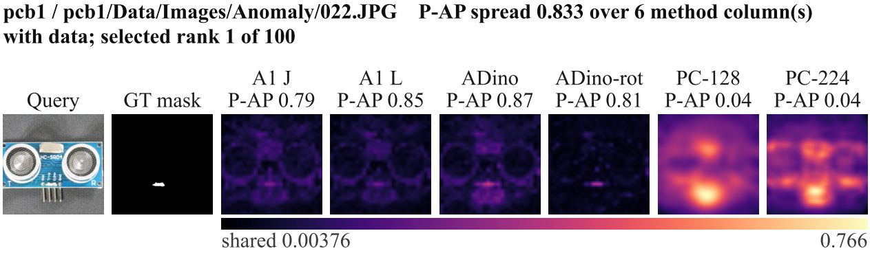
Figure 7 - visa pcb1: multi-method per-sample comparison on the S8 common region (seed 0, K 4; region 392 x 393, 59.8% of the canvas)
