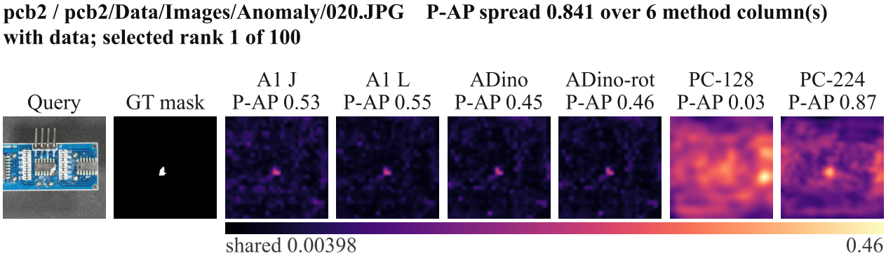
Figure 7 - visa pcb2: multi-method per-sample comparison on the S8 common region (seed 0, K 4; region 392 x 393, 59.8% of the canvas)
