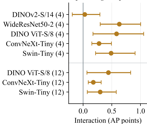
(c) BTAD Equal-weight replacement
