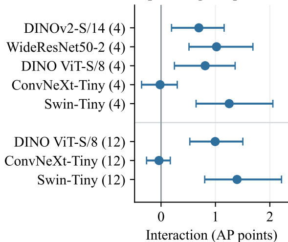
(a) MPDD Equal-weight replacement
