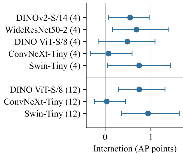
(b) MPDD Balanced replacement
