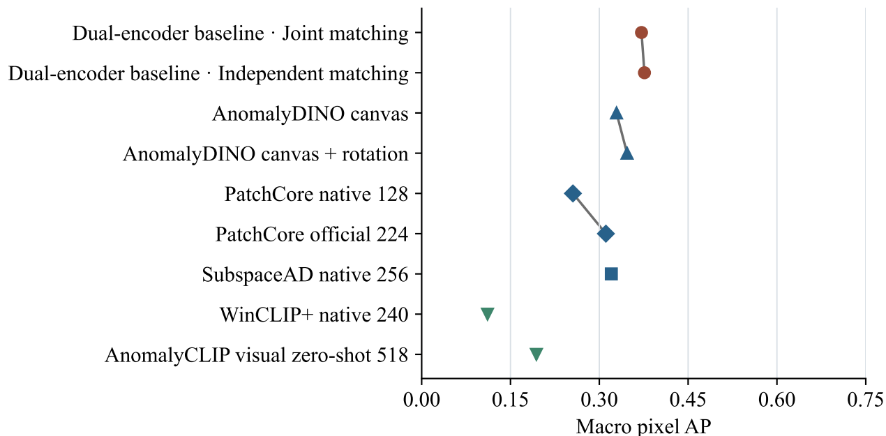
VisA
