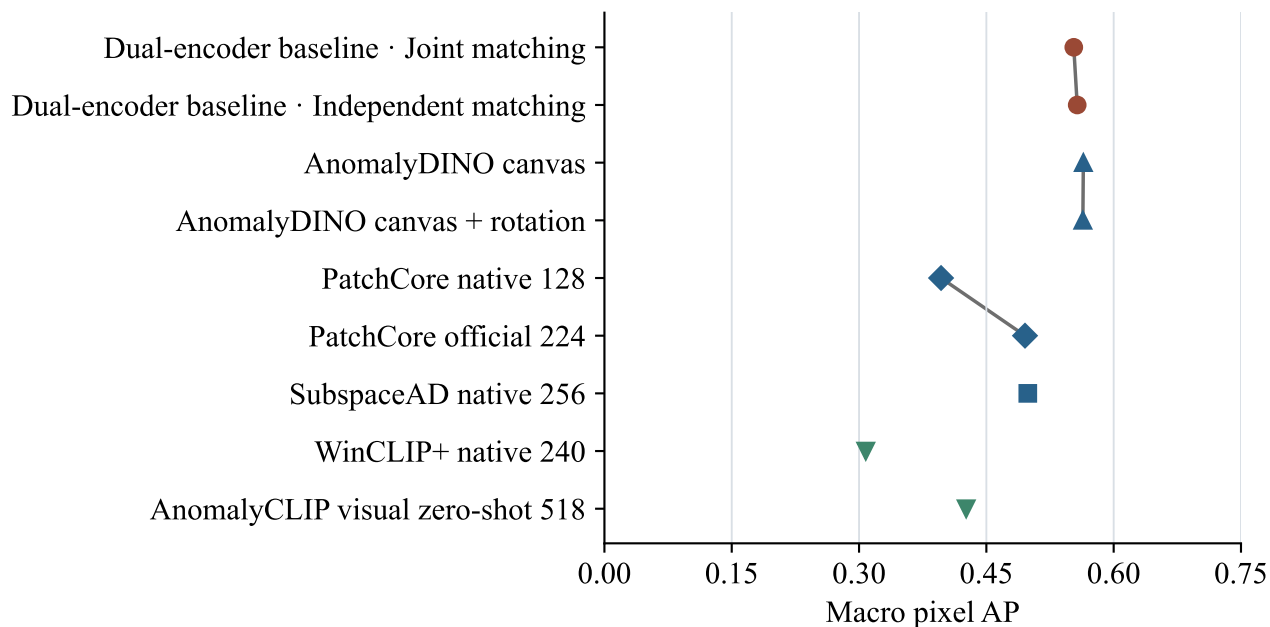
MVTec AD
