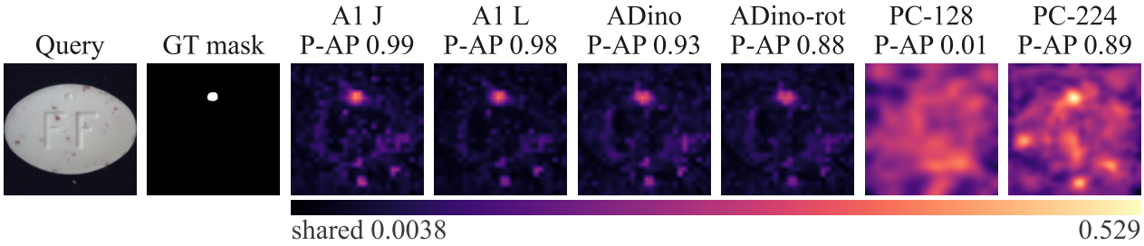
Figure 7 - mvtec pill: multi-method per-sample comparison on the S8 common region (seed 0, K 4; region 392 x 392, 76.6% of the canvas) pill / pill/test/scratch/019.png P-AP spread 0.978 over 6 method column(s) with data; selected rank 1 of 141
