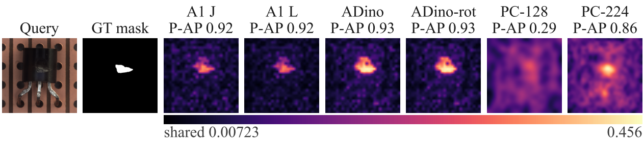
transistor / transistor/test/bent_lead/001.png
