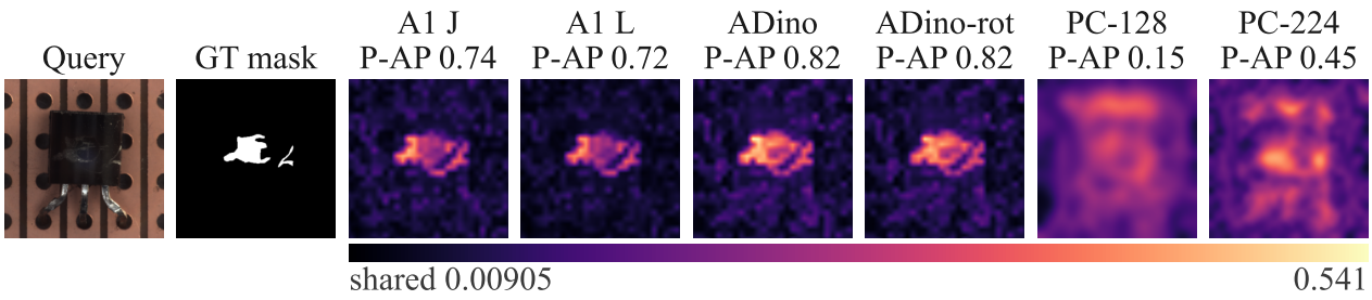
transistor / transistor/test/damaged_case/007.png
