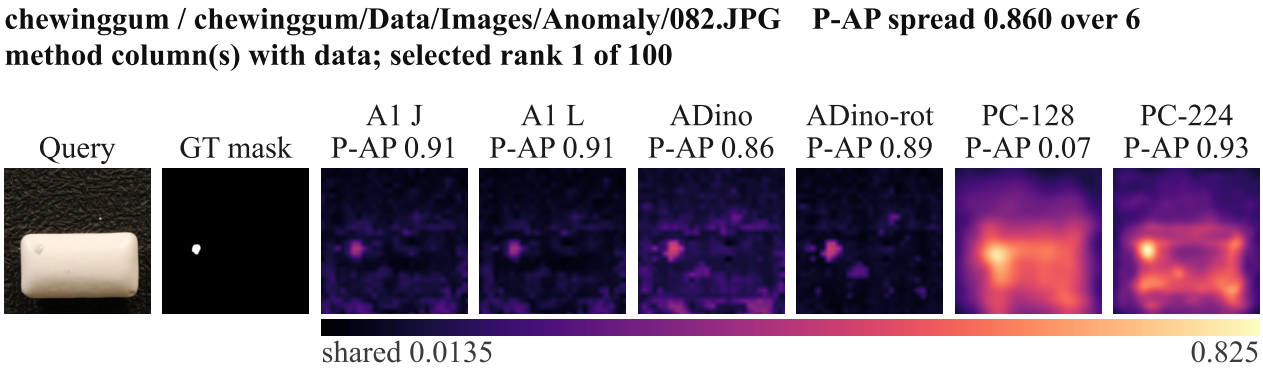
Figure 7 - visa chewinggum: multi-method per-sample comparison on the S8 common region (seed 0, K 4; region 392 x 392, 64.6% of the canvas)
