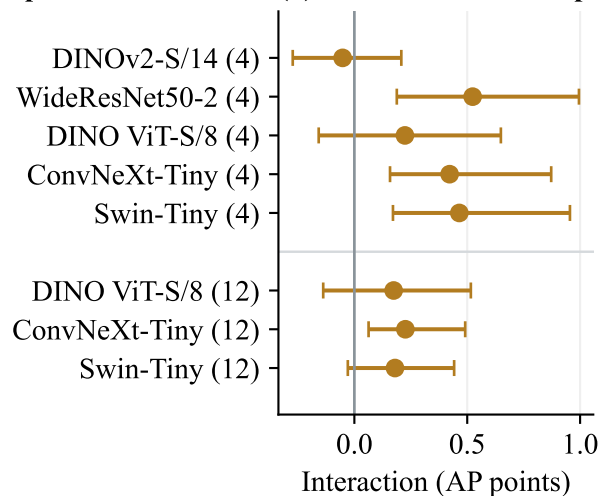
(c) BTAD · Equal-weight replacement
