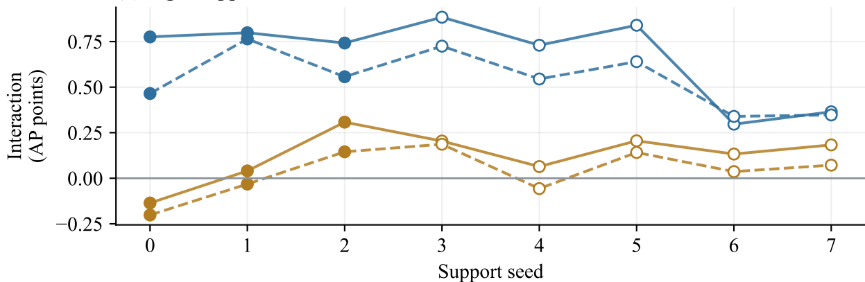
(b) Eight support seeds
