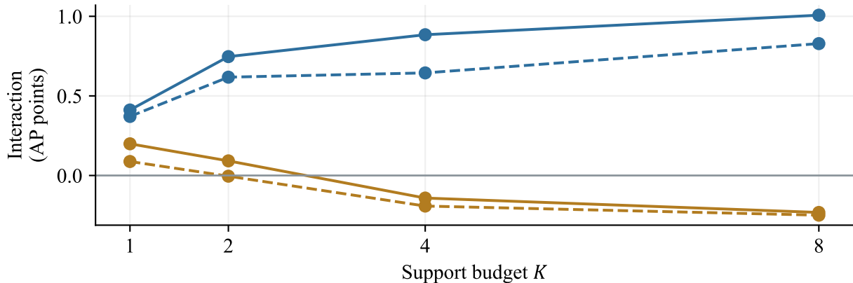
● MPDD Equal-weight replacement ● BTAD Equal-weight replacement - - ● MPDD Balanced replacement - - ● BTAD Balanced replacement (a) Nested support budgets
