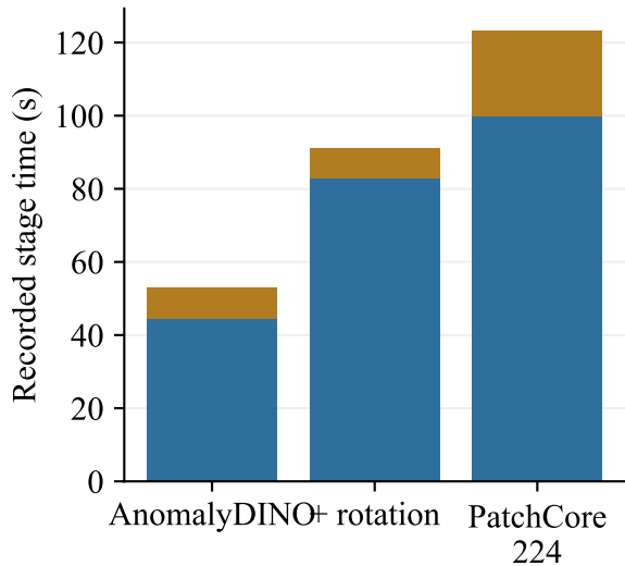
(a) MPDD
