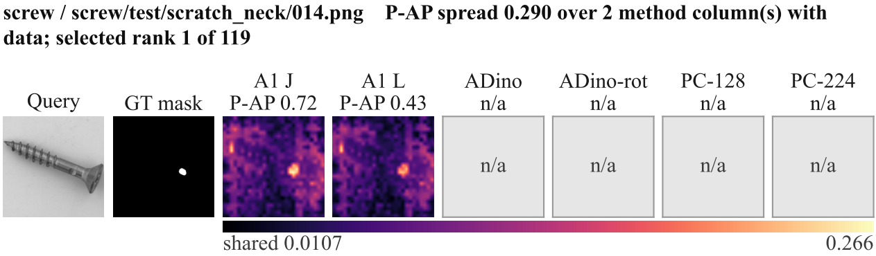
Figure 7 · MVTEC screw · common-region comparison (seed 0, K 4; 392 × 392 grid; 76.6% canvas)
