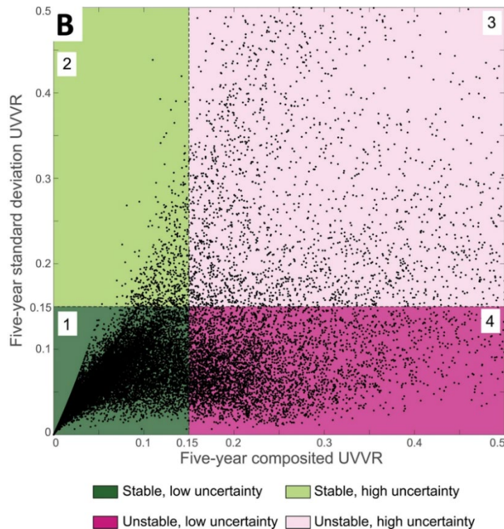
Figure 3. Scatterplot of five-year composited and standard deviation of UVVR, used to identify areas that have crossed the nominal 0.15 stability threshold. 1) Indicates stable, low uncertainty pixels that are consistently below the stability threshold of 0.15 (i.e., good) and don't fluctuate much; 2) indicates stable, high uncertainty pixels that are below the stability threshold of 0.15, but there are big annual outliers (e.g., overwash event, dieback); 3) indicates unstable, high uncertainty pixels that are above the stability threshold of 0.15 (i.e., bad) and there are large annual fluctuations (water levels, controlled burn); and 4) indicates unstable, low uncertainty pixels that are consistently above the stability threshold of 0.15, and they don't fluctuate much (Ganju 2022).
