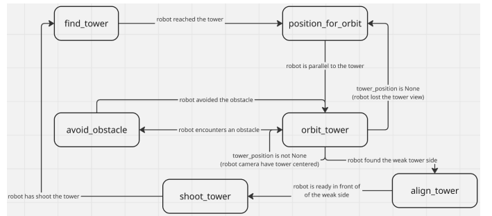
Figure 4: Robot state machine diagram illustrating the tower detection and interaction workflow.
