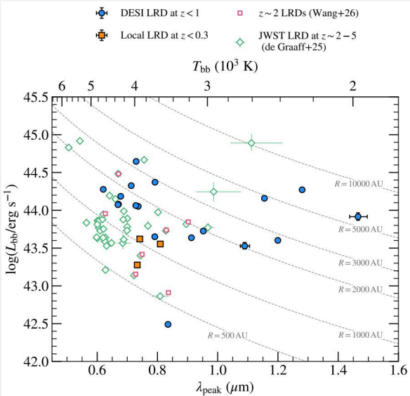
Fig. 4. Several low- z LRDs peak beyond 1 micron, pointing to especially cool, large blackbody-like envelopes that high- z samples rarely populated.
