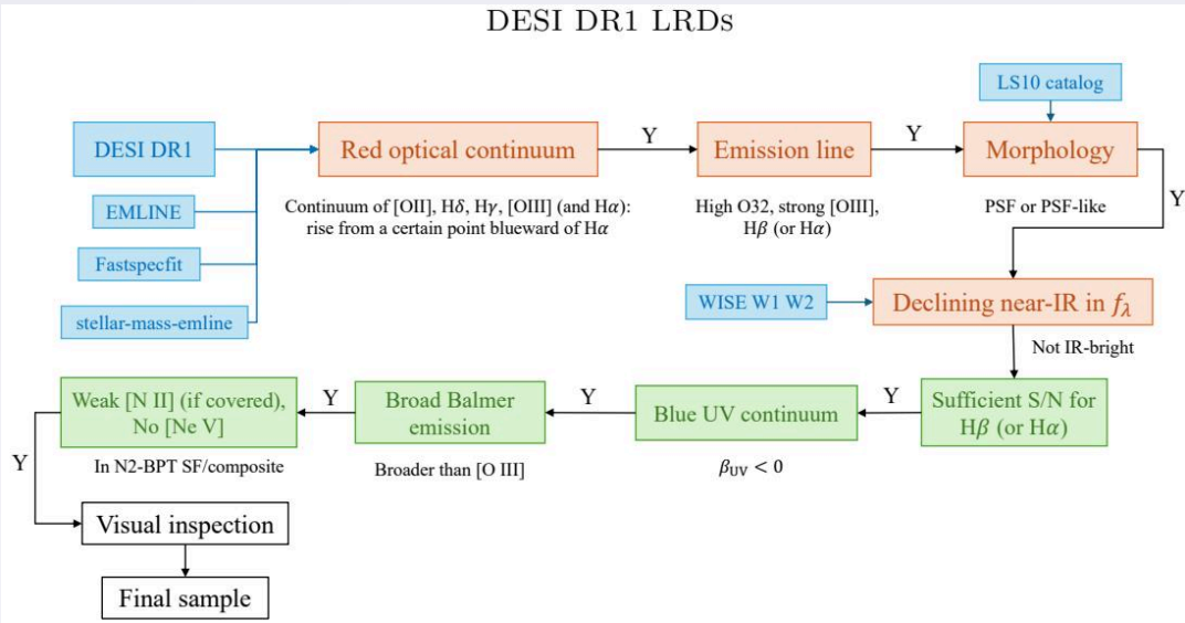
Fig. 1. A conservative pipeline: candidates had to pass continuum, line, morphology, UV, and broad-Balmer tests before entering the final sample.
