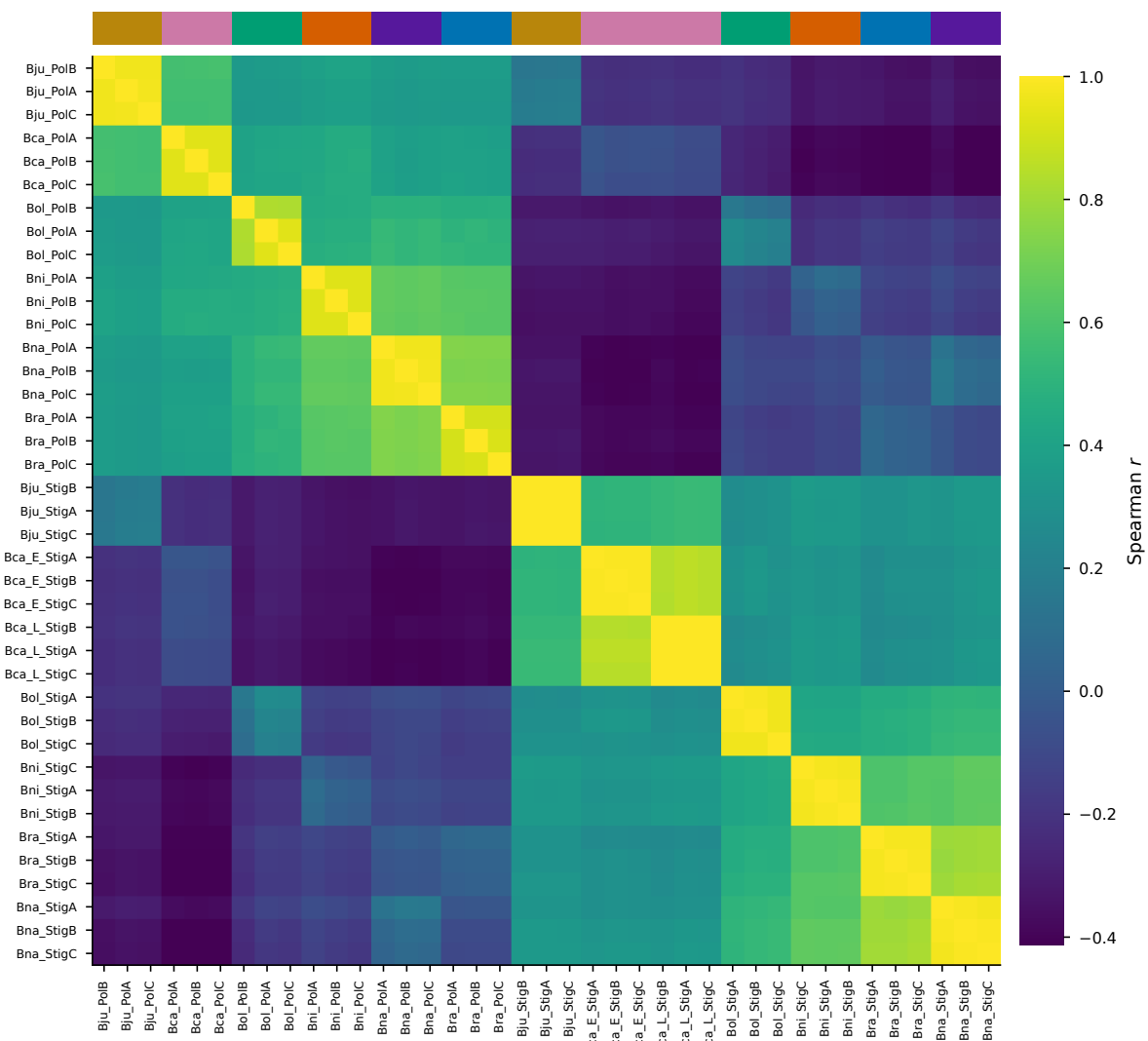
library correlation, hierarchically clustered; the strip marks species
