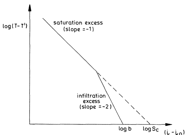
FIG. 7. Expected nature of results from infiltrometer experiments interpreted in terms of the storage based infiltration component of the model.
