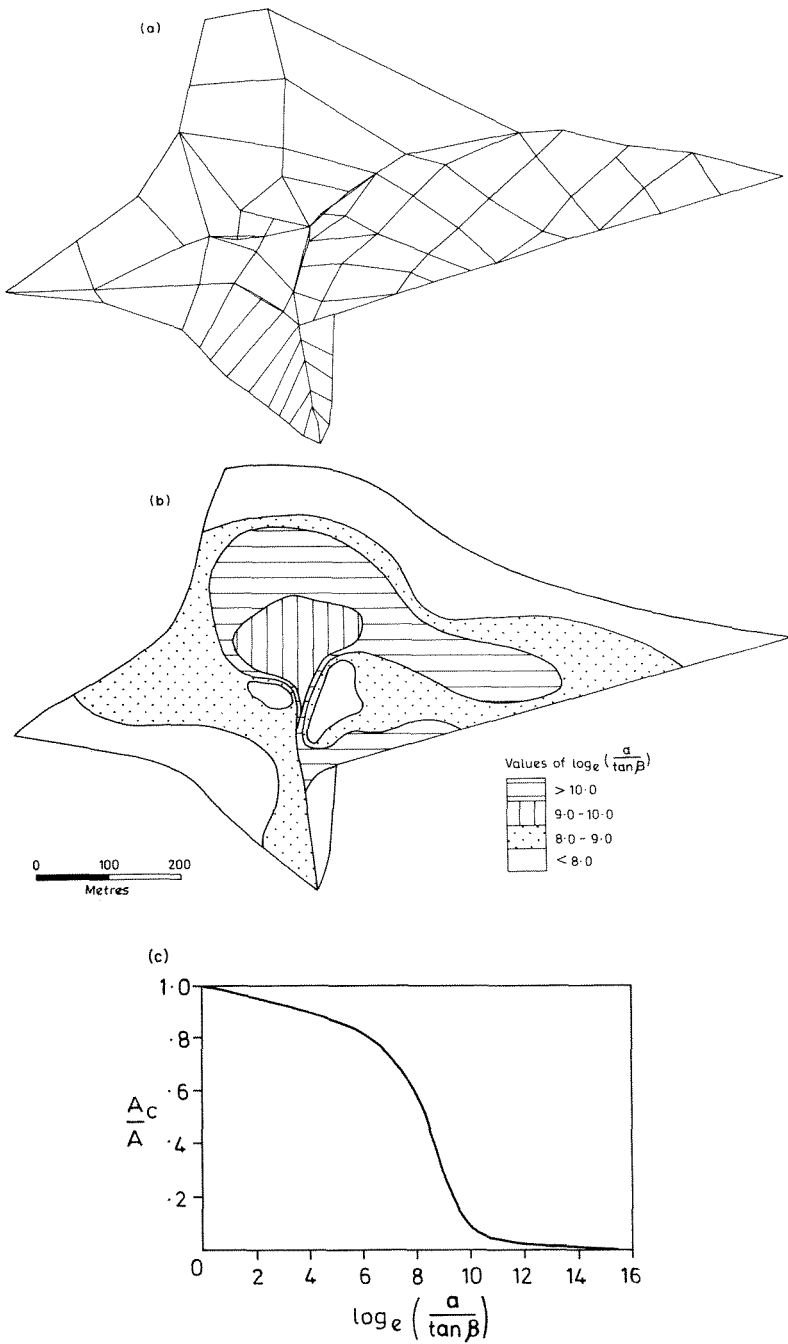
FIG. 4(a) The discretization of the Lanshaw sub-basin (area 1A). (b) The spatial distribution of calculated values of \ln(a/\tan \beta) in the Lanshaw sub-basin. (c) The cumulative distribution of contributing area A_c exceeding given value of \ln(a/\tan \beta) for the Lanshaw sub-basin.
