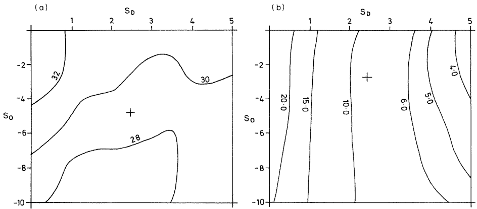
FIG. 15. (a) F_1 response surface for the parameters S_D and S_0 . Lanshaw sub-basin, November/December 1974 simulation. Cross represents estimated values. (b) F_1 response surface for the parameters S_D and S_0 . Lanshaw sub-basin, March/April 1975 simulation. Cross represents estimated values.
