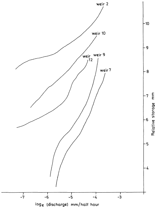
FIG. 8. Recession curves for different sites in the Crimple Beck basin as storage/ \ln (discharge) plots.
