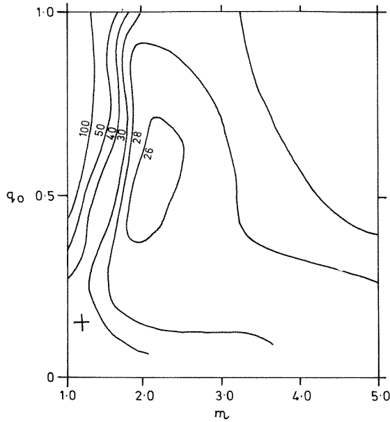
FIG. 14. F_1 response surface for the parameters m and q_0 . Lanshaw sub-basin November/December 1974 simulation. Cross represents estimated values.
