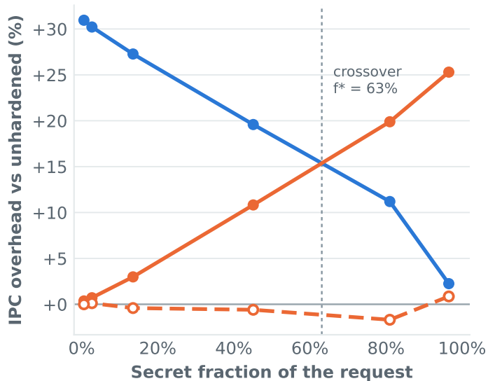
gem5 Neoverse-V2 FDP (EVES + VTAGE)
