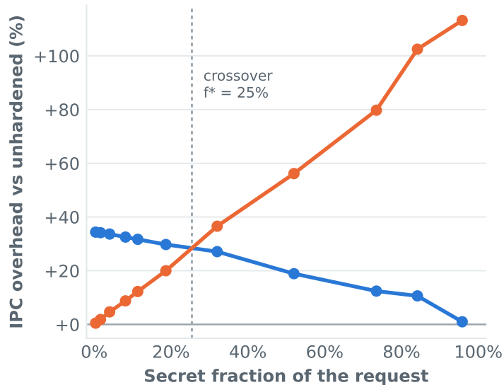
Apple M4 (load value predictor, 36-bit)
