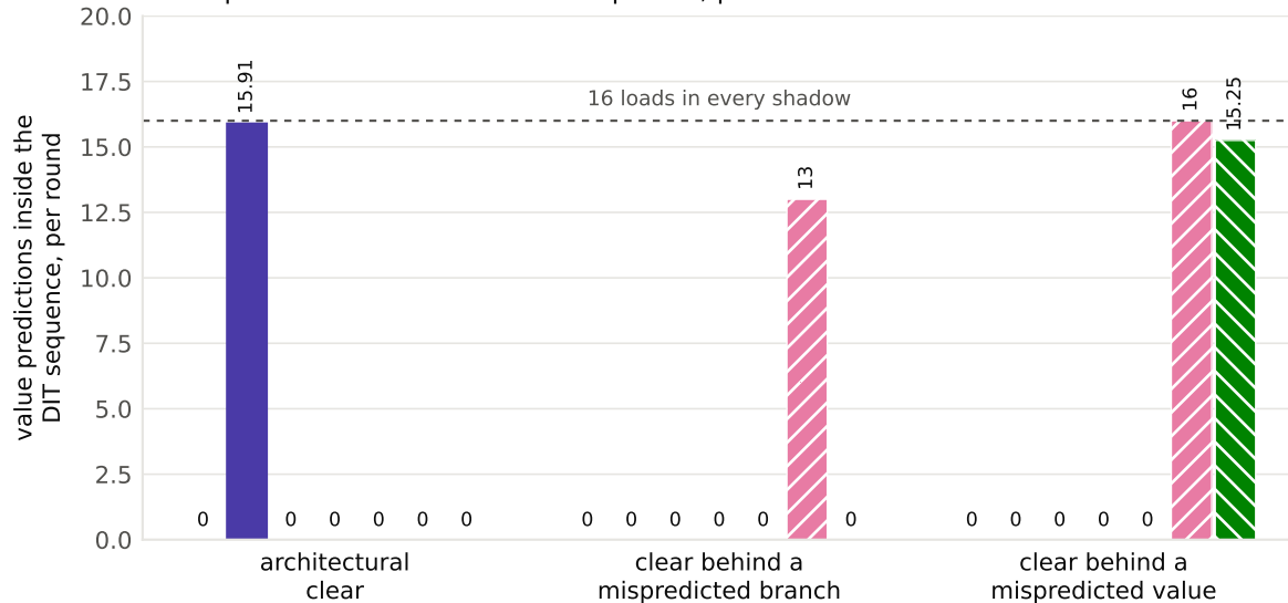
Value predictions inside the DIT sequence, per round
