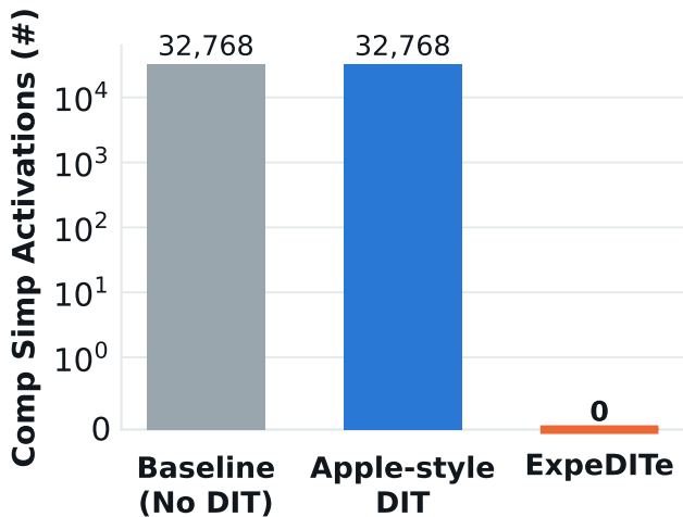
(c) Computation Simplification
