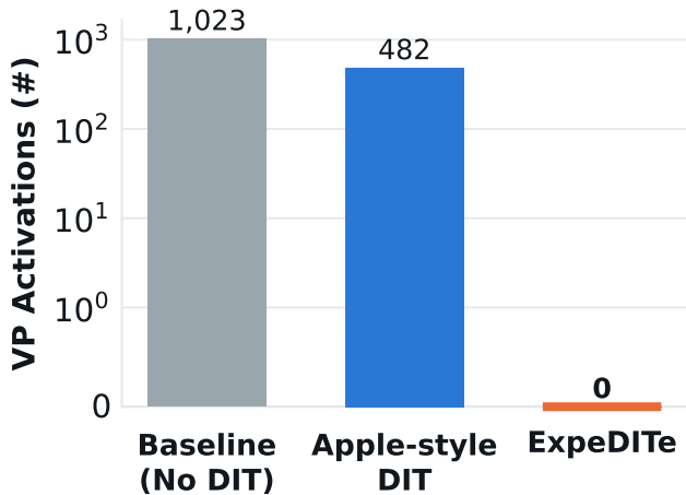
(a) Value Prediction
