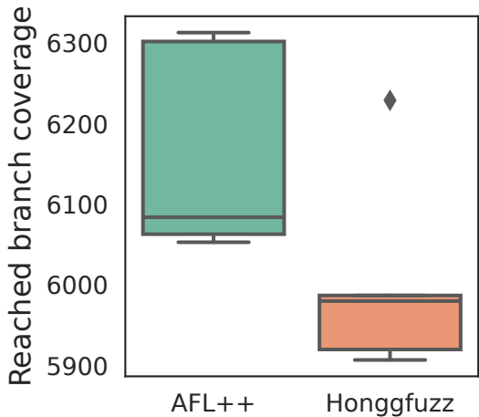
(a) bloaty_fuzz_target
