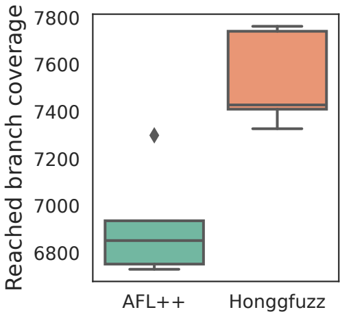
(b) proj4_proj_crs_to_crs_fuzz
