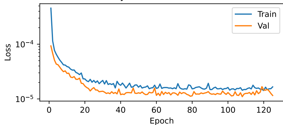
Attention Position Loss
