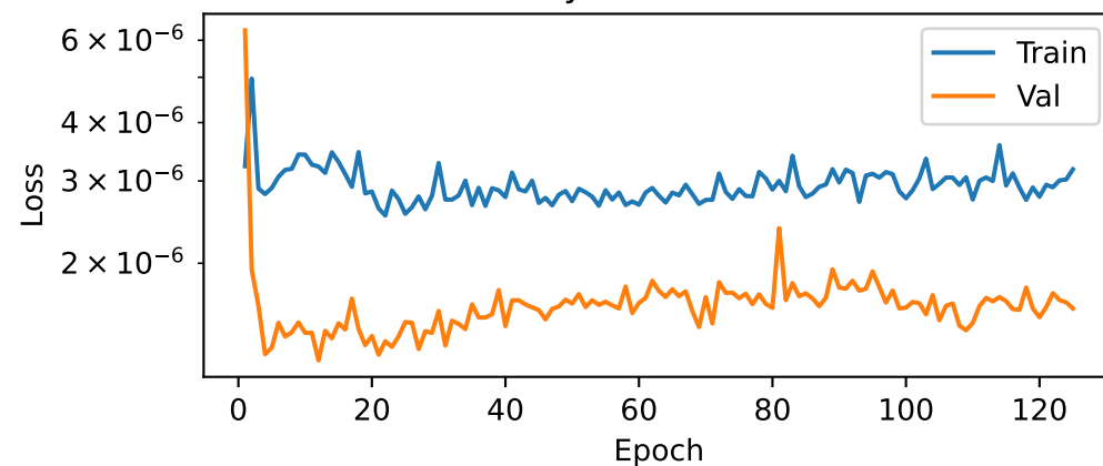
Steady State Loss
