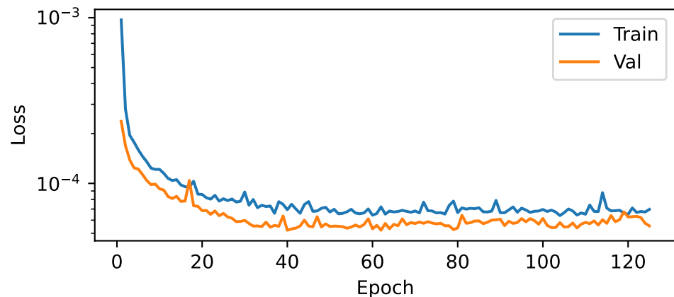
Dynamic Recon Loss
