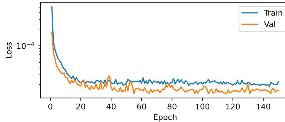
Dynamic Loss
