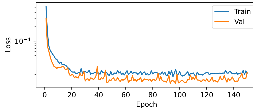
Dynamic Loss
