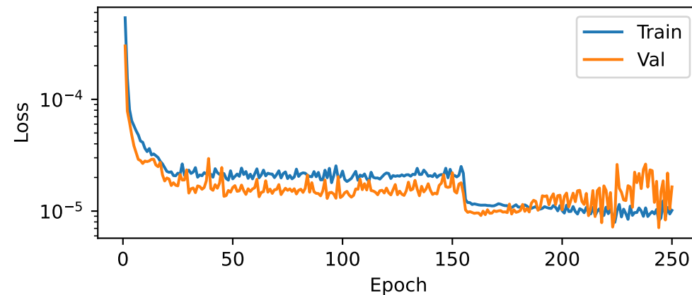
Dynamic Loss
