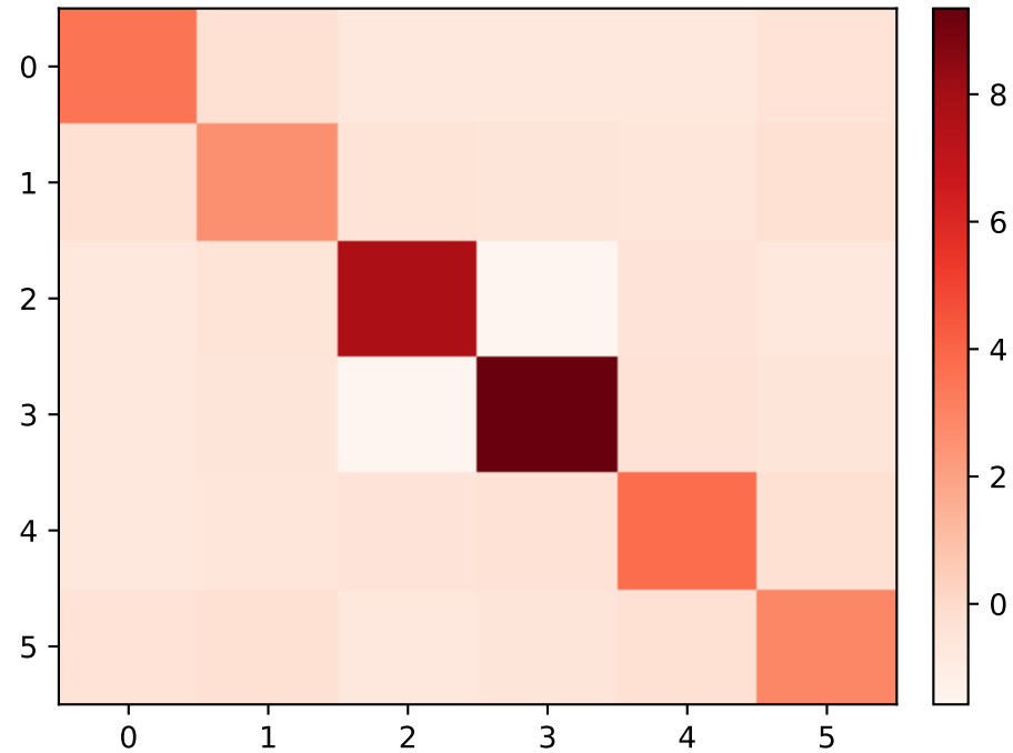
Stiffness Matrix (K)
