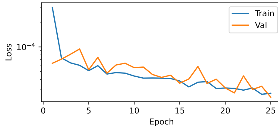
Dynamic Loss
