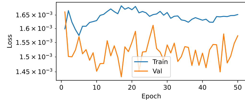
Attention Consistency Loss
