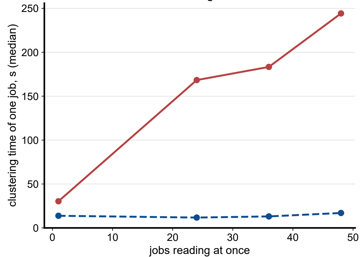
Clustering time
