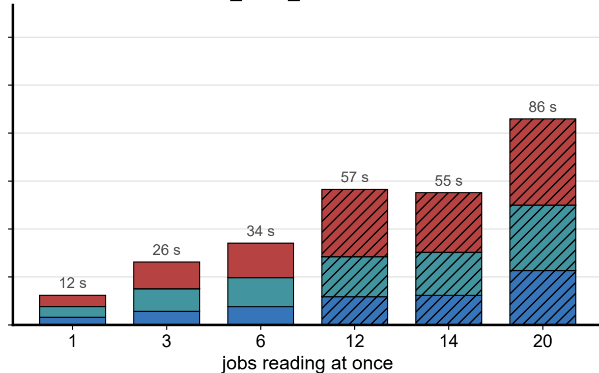
OMP_NUM_THREADS = 1
