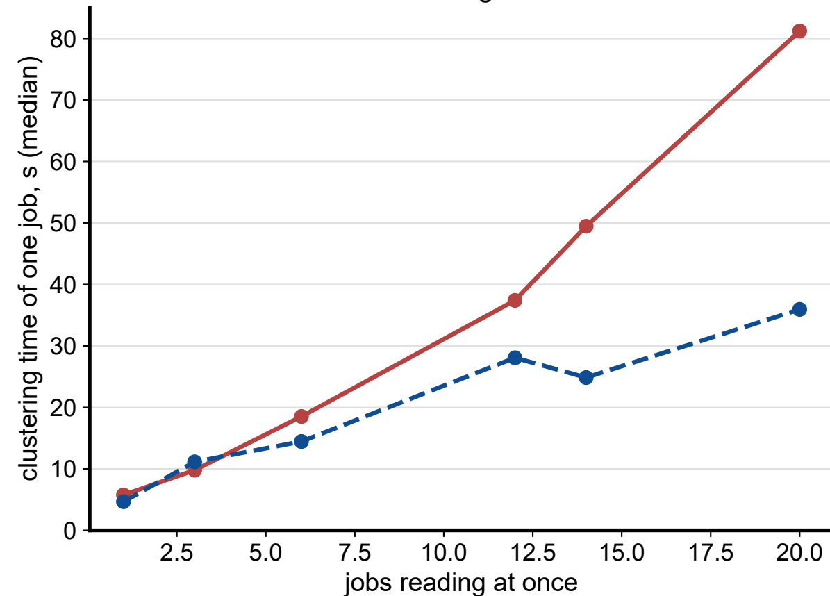
Clustering time
