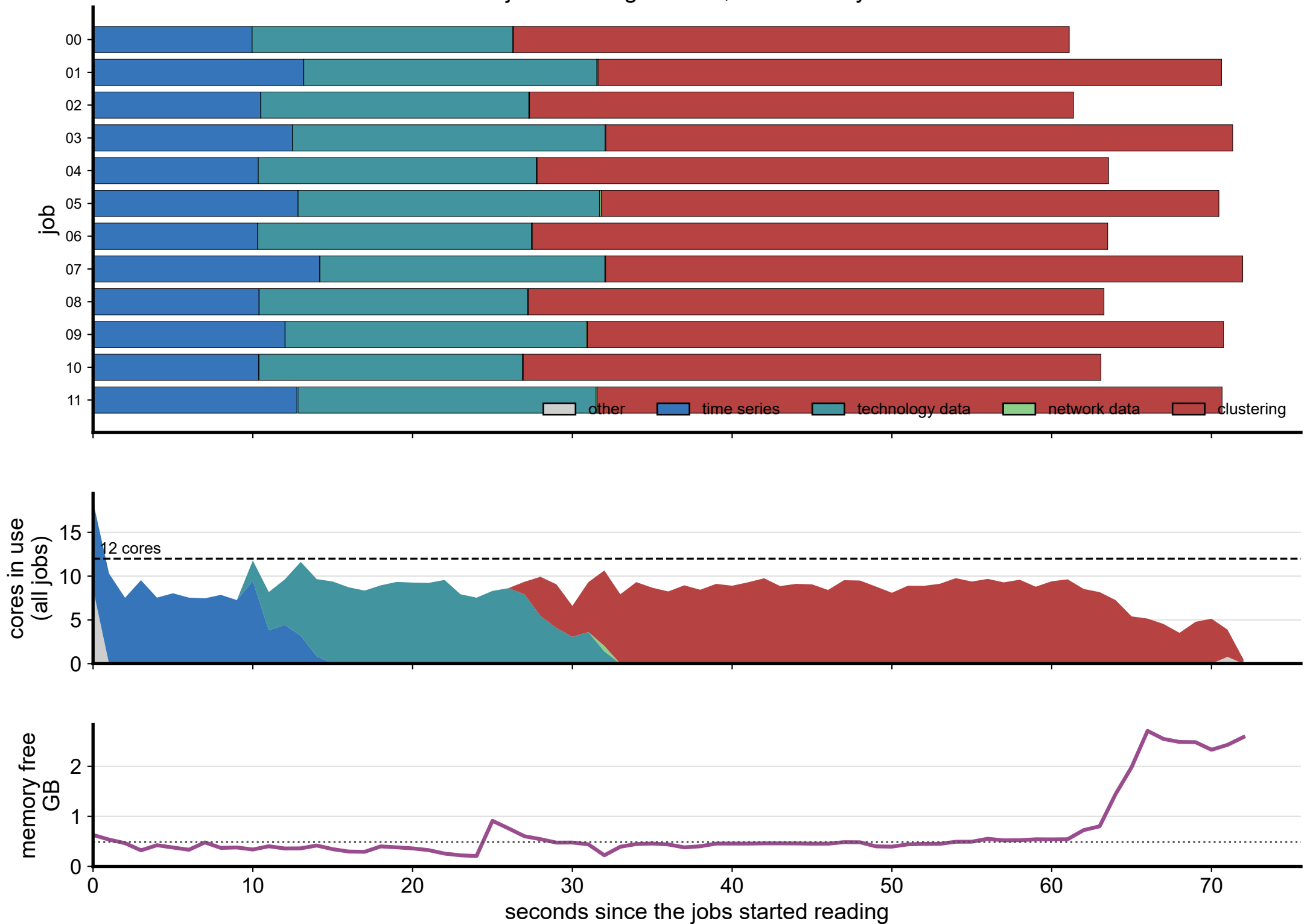
12 jobs reading at once, as the study runs
