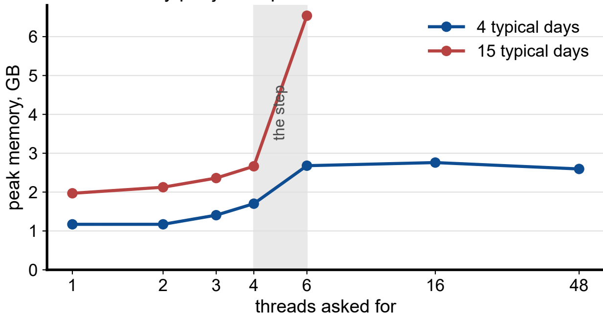
Memory per job steps between four and six threads
