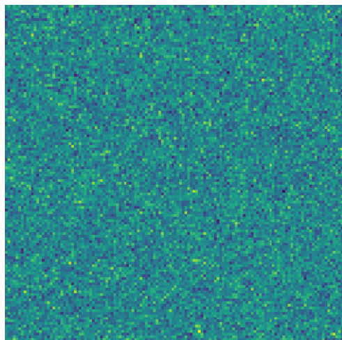
Cosmo3DFlow
