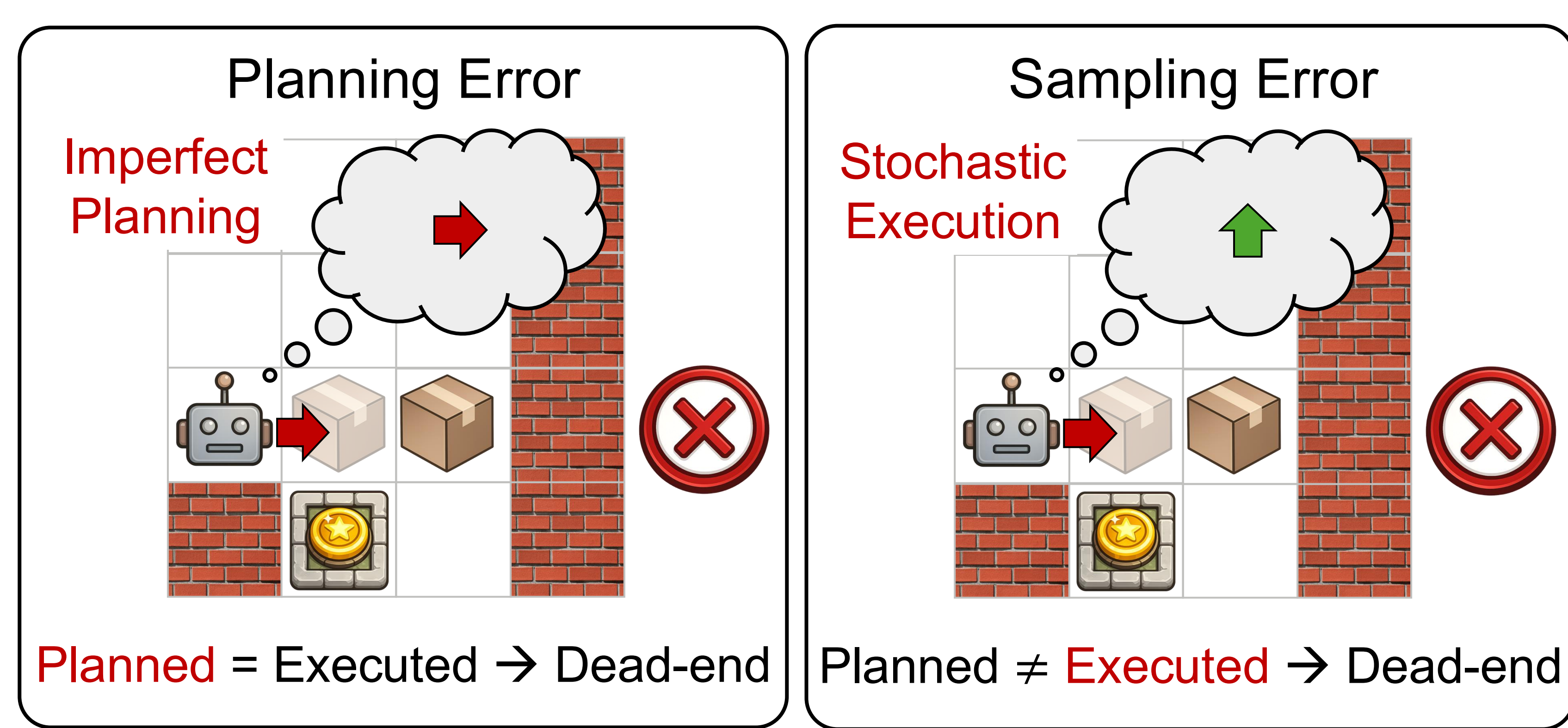
(a) Sources of Irrecoverable Failures in the ReAct Framework
