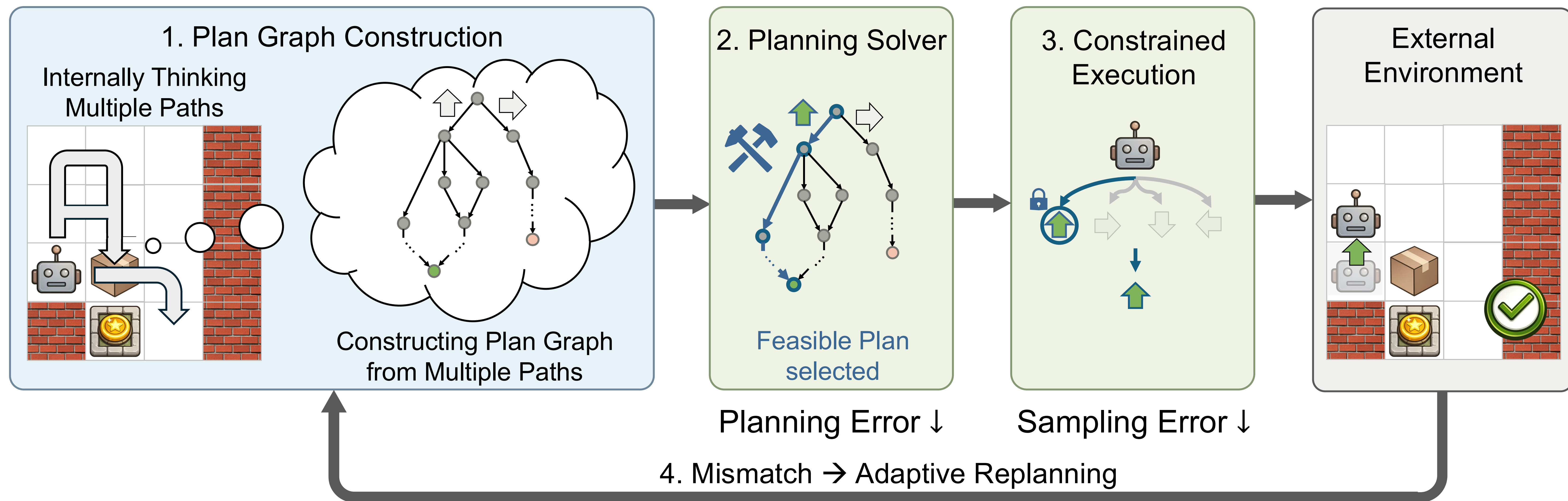
(c) Our Framework: Tool-guided Adaptive Planning with constrained Execution (TAPE)
