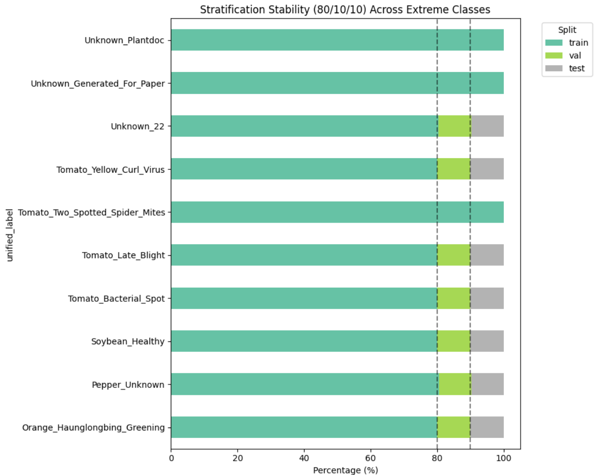
Figure: GroupKFold Stratified Split Verification without Data Leakage
