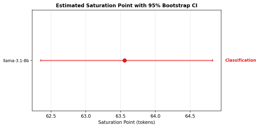
Figure 6: Saturation point estimate for classification with 95% bootstrap confidence interval. The narrow interval indicates that the saturation estimate is stable across resampled evaluation sets.
