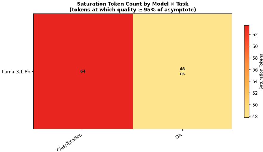
Figure 5: Estimated saturation token counts for the replication experiment. Classification saturates at approximately 64 tokens, while no statistically significant saturation point is detected for question answering.
