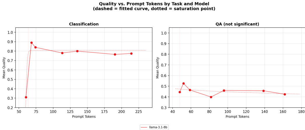
Figure 4: Replication experiment using 200 examples. Sentiment classification exhibits a clear saturation pattern, with performance rapidly increasing and then plateauing as prompt tokens increase. In contrast, question answering shows no systematic improvement with longer prompts.
