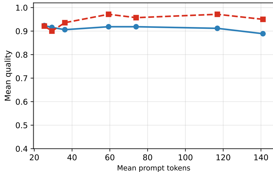
QA (curve-shape r = 0.10 )
