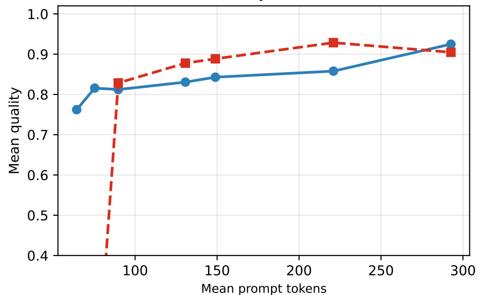
Math reasoning (curve-shape r = 0.52 )
