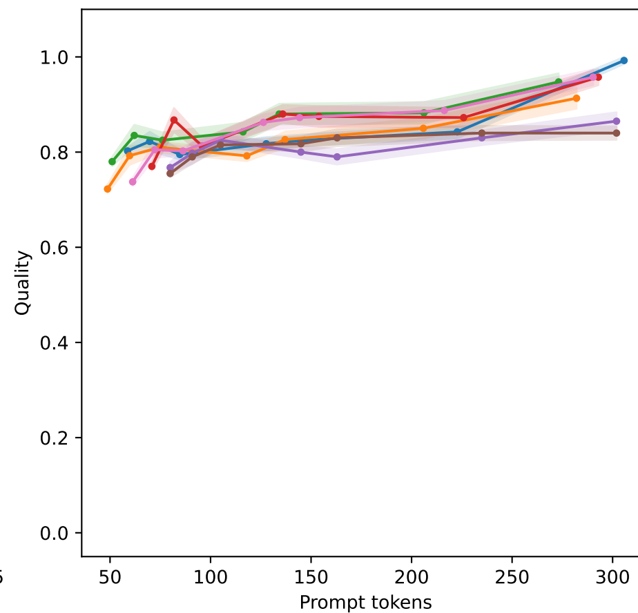
Math Reasoning
