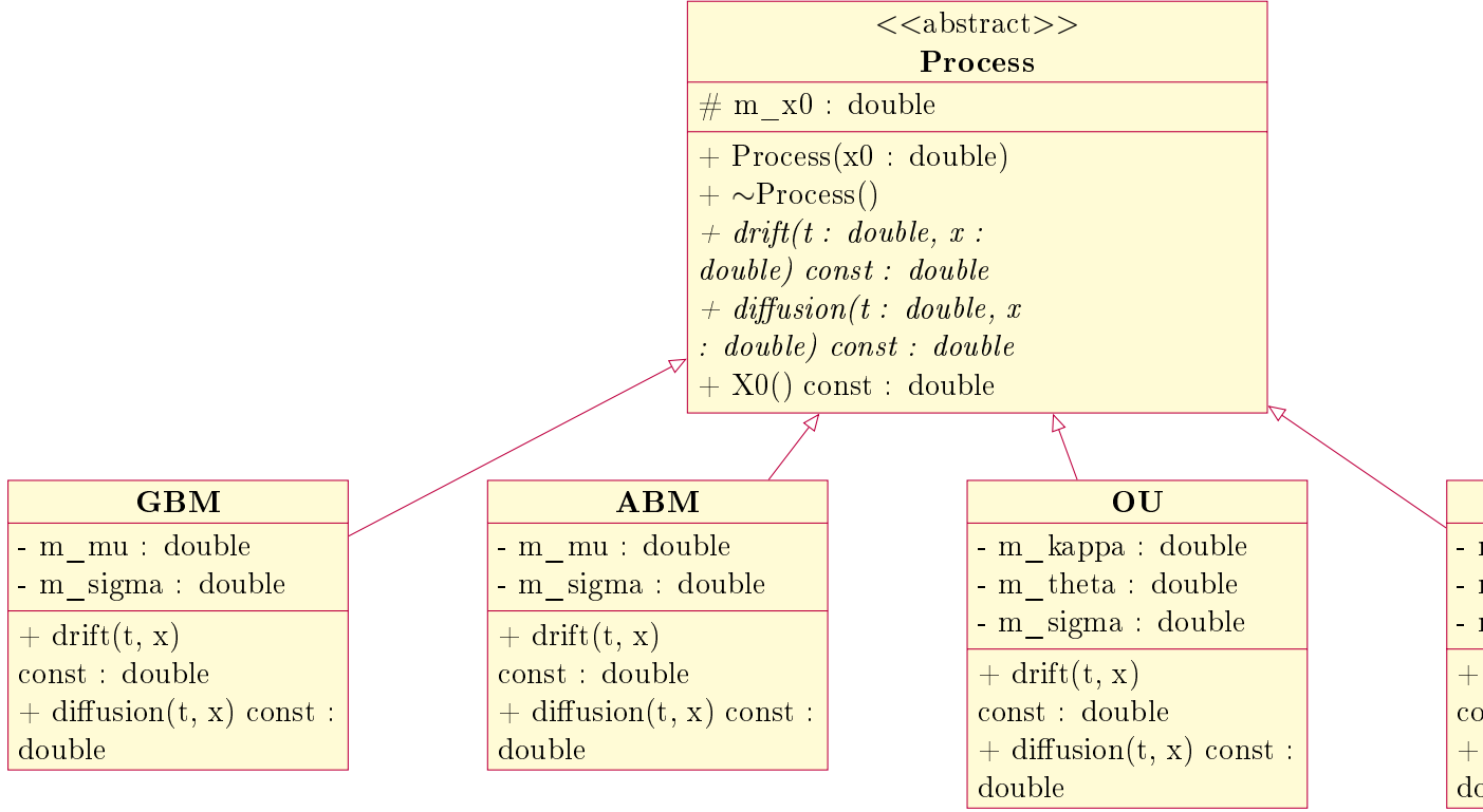
Figure 1: The Process hierarchy. Abstract operations ( italic ) are the interface consumed by both the exact samplers of ???? and the numerical schemes below.
