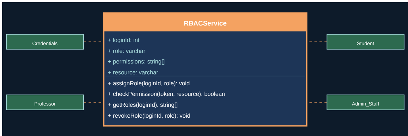
Figure 5.1 - UML Class Diagram
