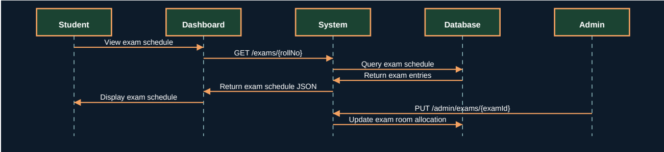
Figure 14.2 - UML Sequence Diagram
