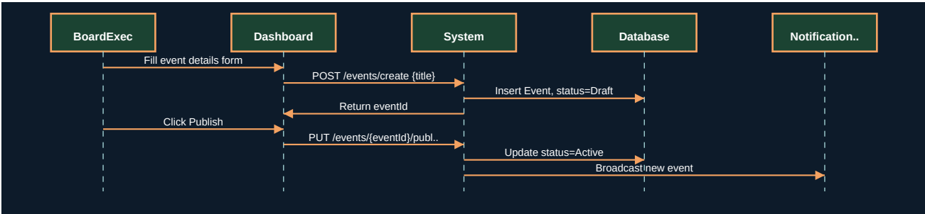
Figure 18.2 - UML Sequence Diagram
