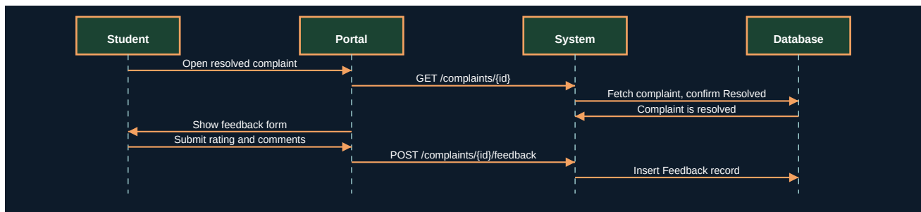
Figure 35.2 - UML Sequence Diagram
