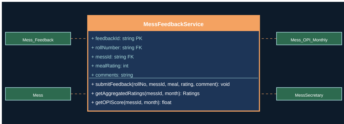
Figure 27.1 - UML Class Diagram
