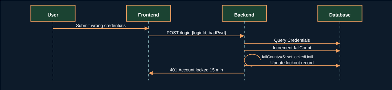
Figure 4.2 - UML Sequence Diagram
