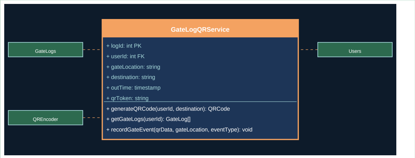
Figure 21.1 - UML Class Diagram
