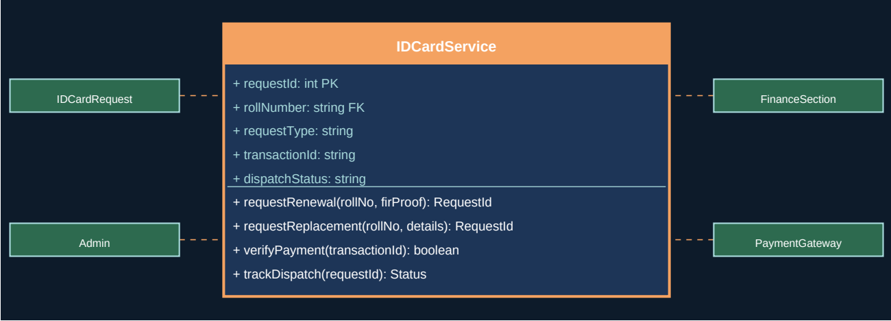
Figure 10.1 - UML Class Diagram
