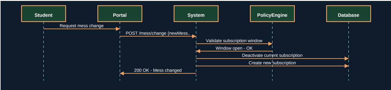
Figure 25.2 - UML Sequence Diagram
