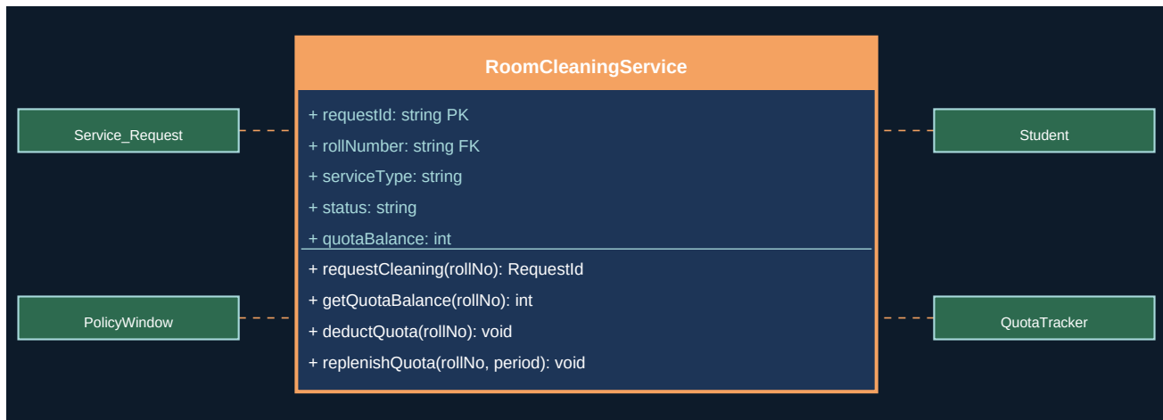
Figure 30.1 - UML Class Diagram
