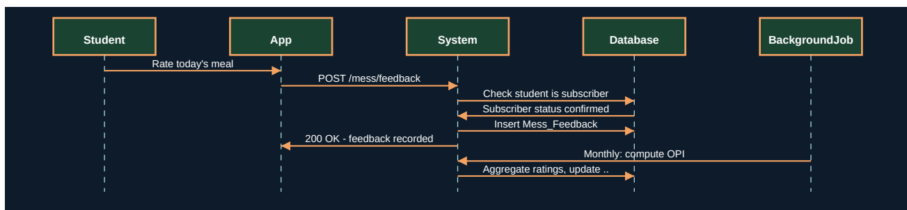
Figure 27.2 - UML Sequence Diagram
