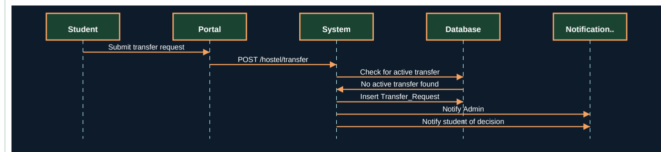
Figure 24.2 - UML Sequence Diagram
