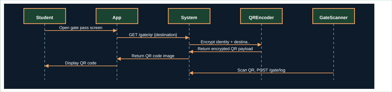
Figure 21.2 - UML Sequence Diagram
