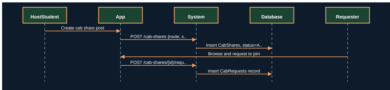
Figure 22.2 - UML Sequence Diagram
