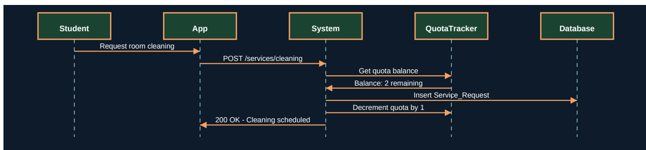
Figure 30.2 - UML Sequence Diagram
