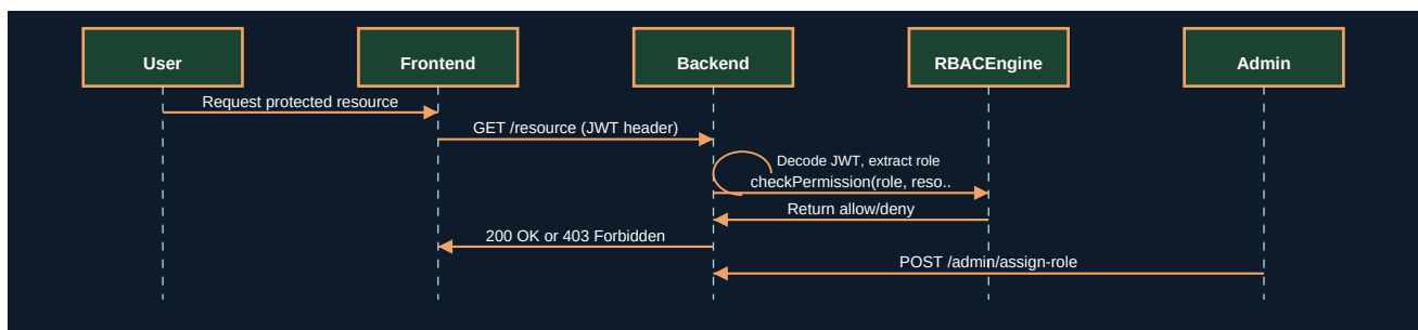
Figure 5.2 - UML Sequence Diagram
