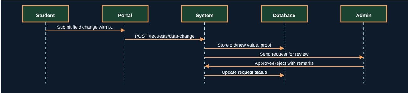
Figure 8.2 - UML Sequence Diagram
