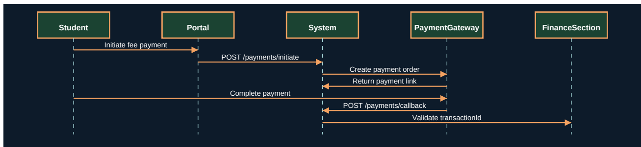
Figure 11.2 - UML Sequence Diagram
