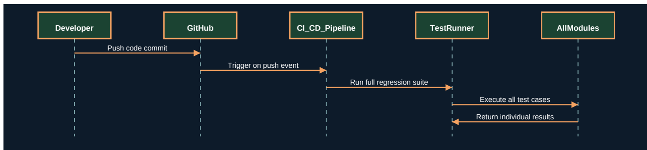
Figure 40.2 - UML Sequence Diagram
