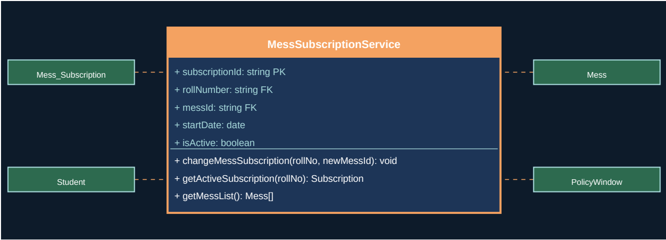
Figure 25.1 - UML Class Diagram
