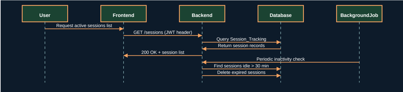
Figure 3.2 - UML Sequence Diagram
