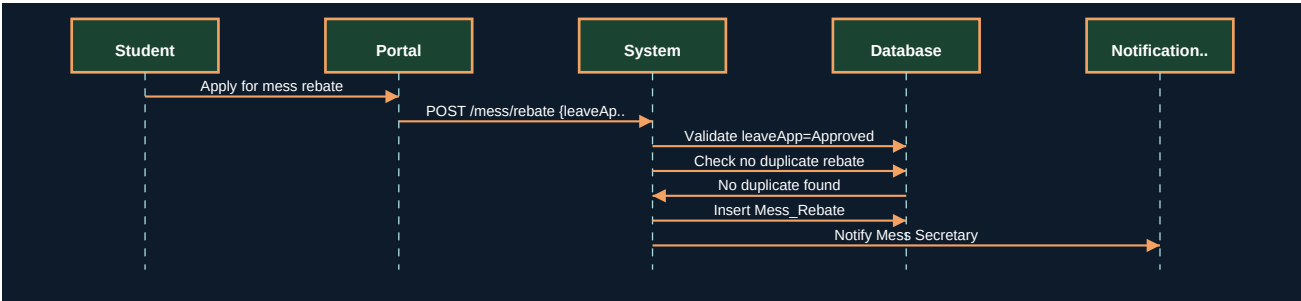
Figure 26.2 - UML Sequence Diagram
