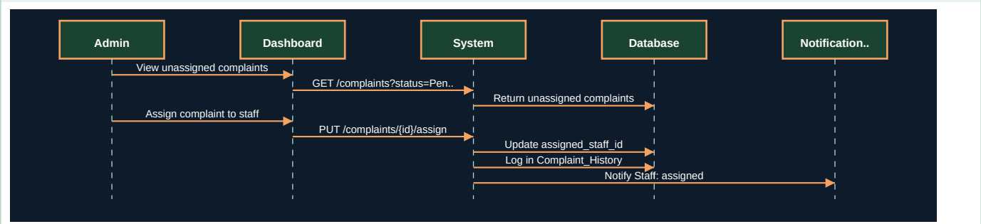
Figure 32.2 - UML Sequence Diagram
