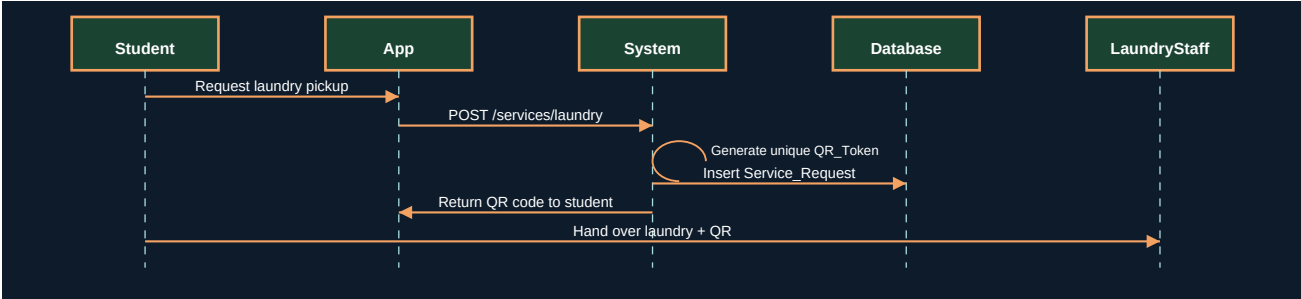
Figure 28.2 - UML Sequence Diagram
