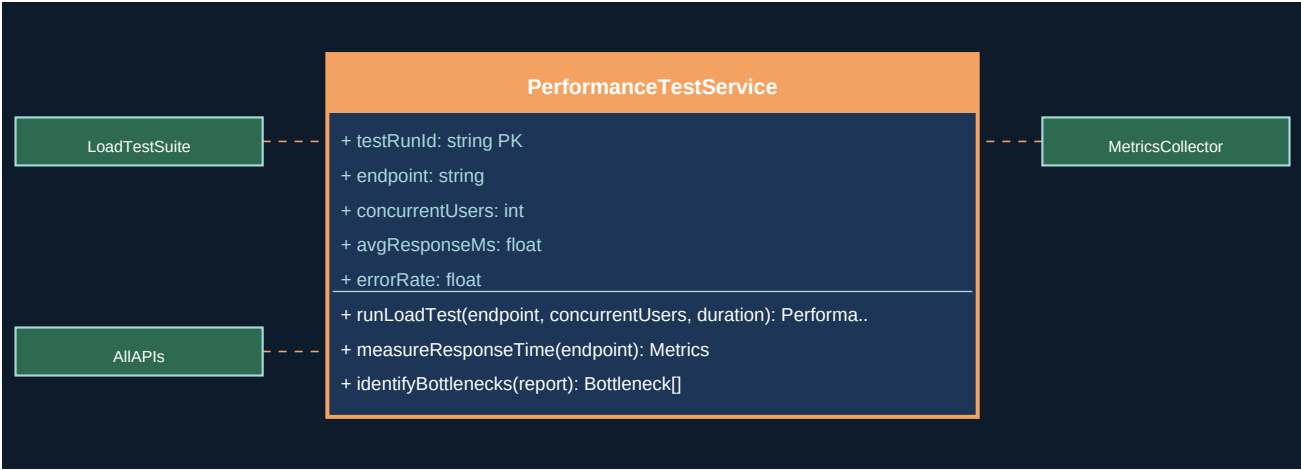
Figure 38.1 - UML Class Diagram
