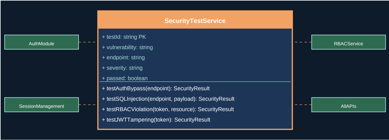
Figure 39.1 - UML Class Diagram
