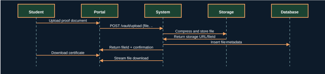
Figure 15.2 - UML Sequence Diagram
