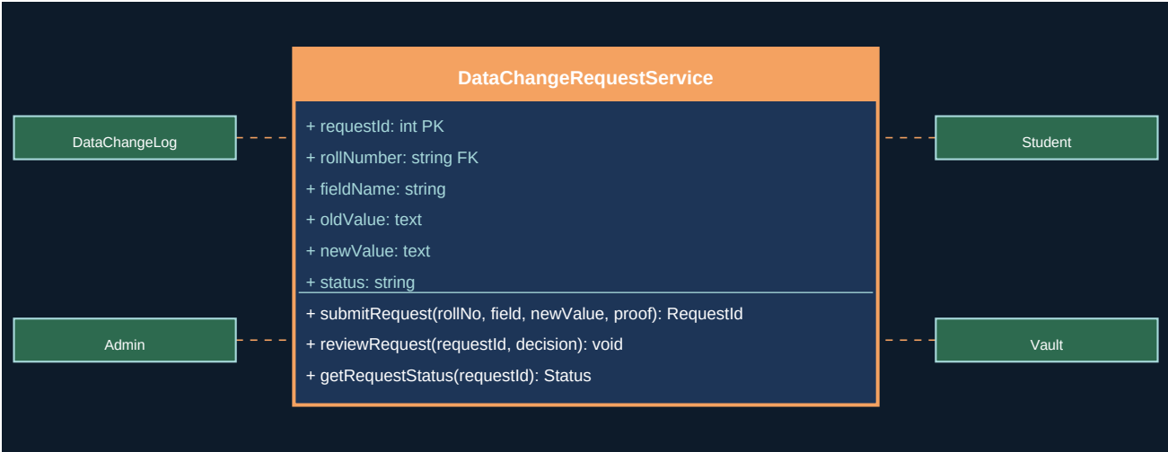
Figure 8.1 - UML Class Diagram
