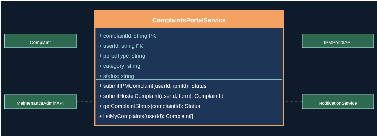
Figure 20.1 - UML Class Diagram
