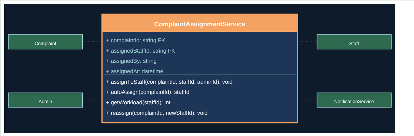
Figure 32.1 - UML Class Diagram
