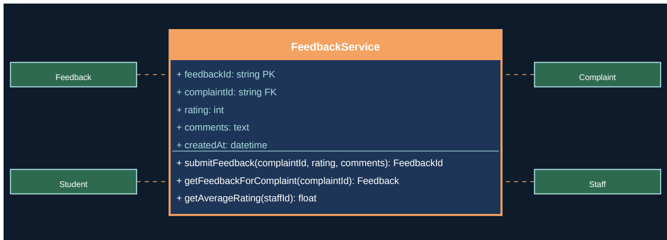
Figure 35.1 - UML Class Diagram
