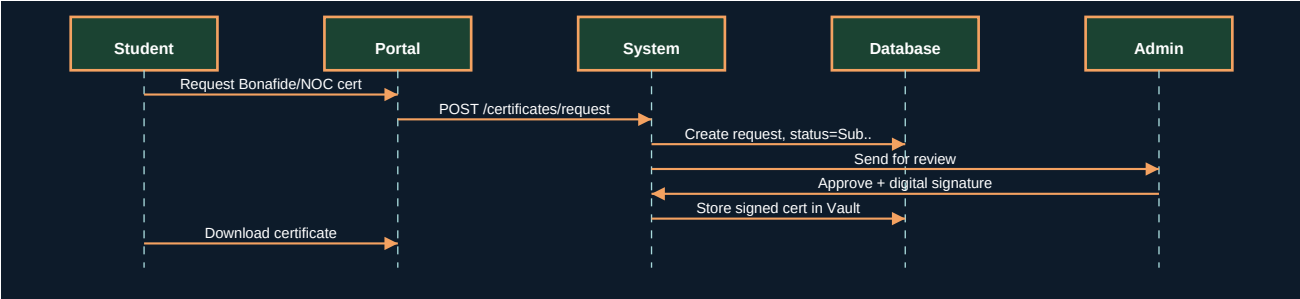
Figure 9.2 - UML Sequence Diagram
