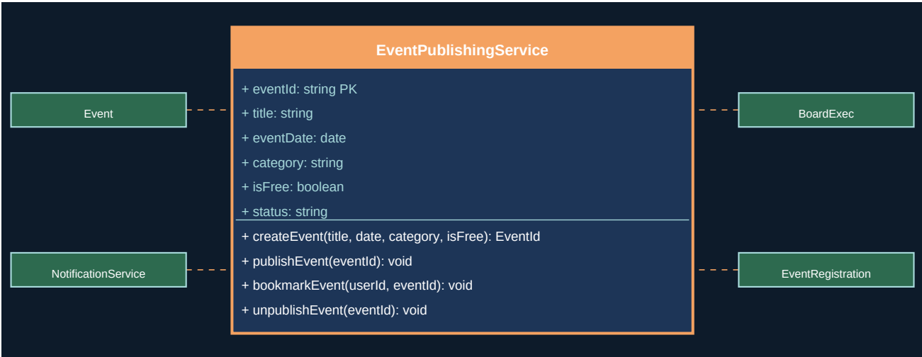
Figure 18.1 - UML Class Diagram
