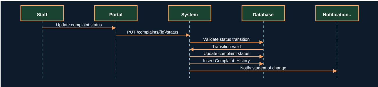
Figure 34.2 - UML Sequence Diagram
