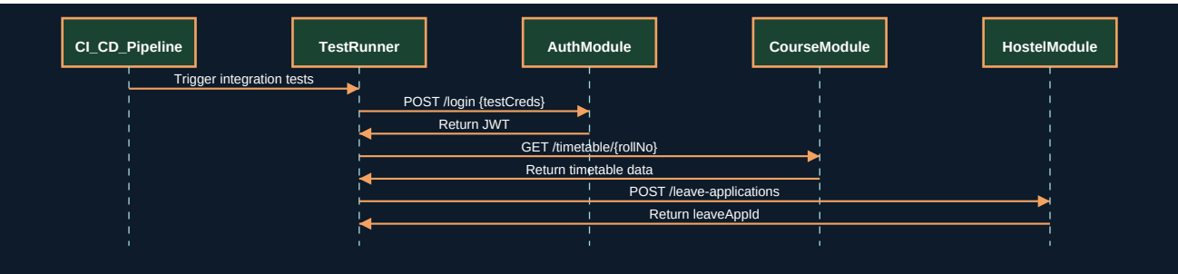
Figure 36.2 - UML Sequence Diagram
