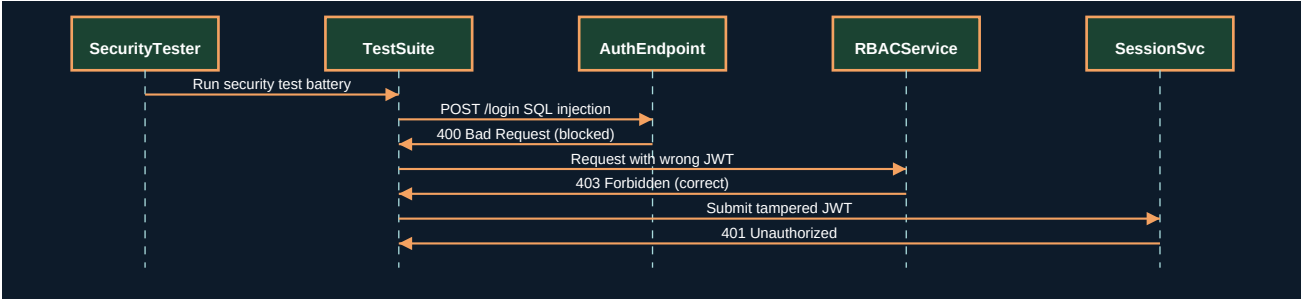
Figure 39.2 - UML Sequence Diagram
