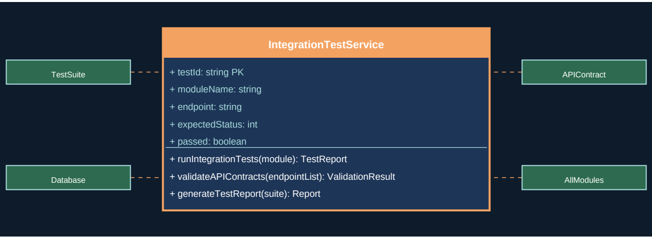
Figure 36.1 - UML Class Diagram
