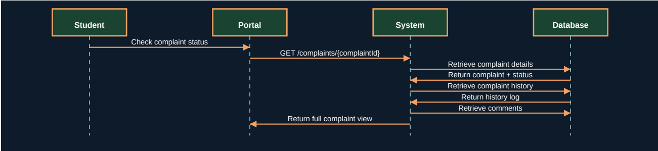
Figure 33.2 - UML Sequence Diagram
