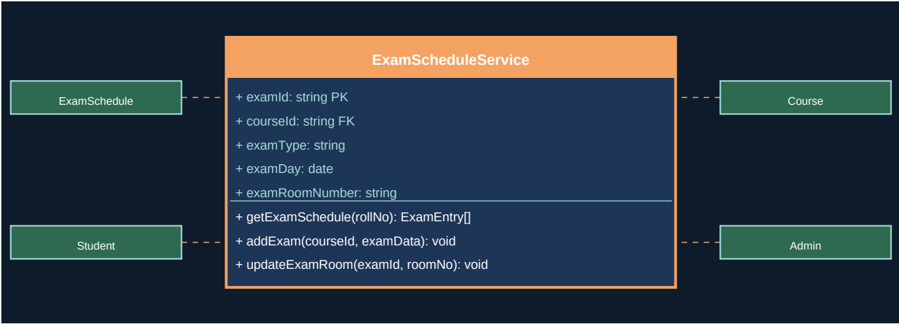
Figure 14.1 - UML Class Diagram
