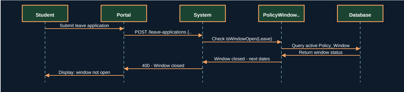
Figure 29.2 - UML Sequence Diagram
