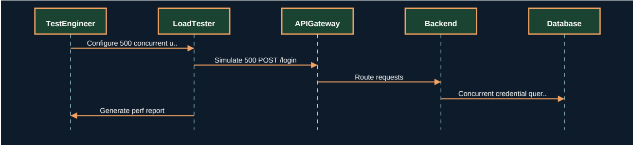
Figure 38.2 - UML Sequence Diagram
