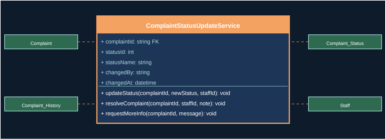
Figure 34.1 - UML Class Diagram
