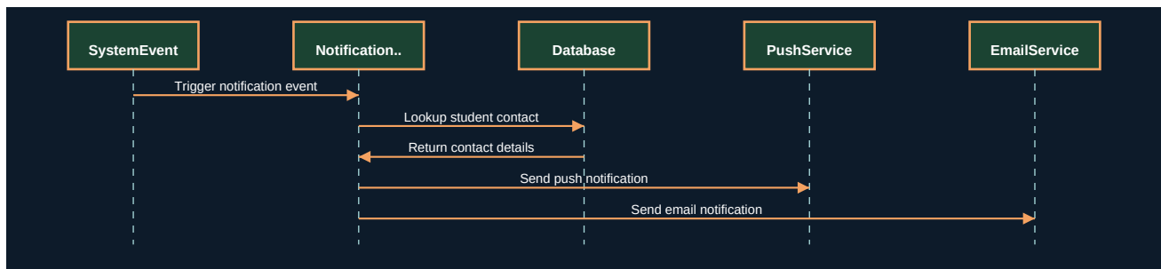
Figure 16.2 - UML Sequence Diagram
