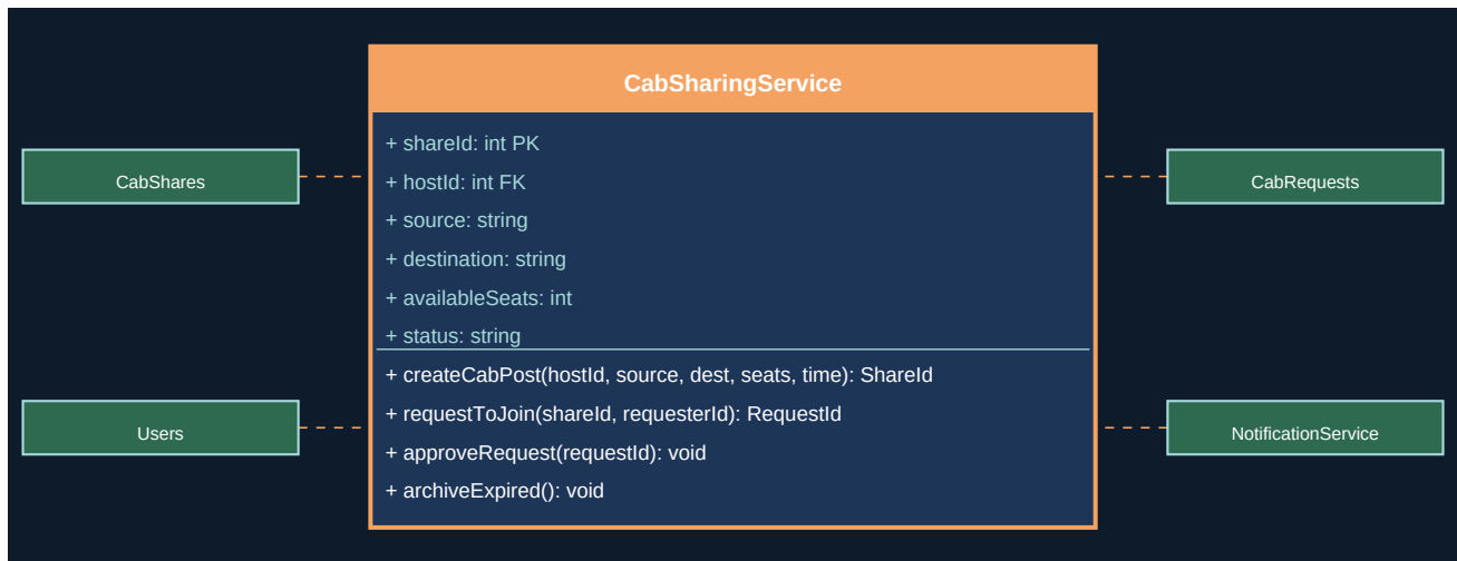
Figure 22.1 - UML Class Diagram
