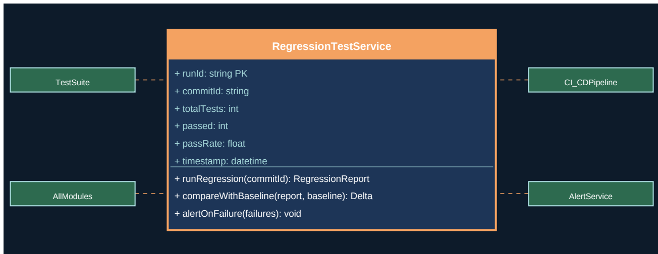
Figure 40.1 - UML Class Diagram
