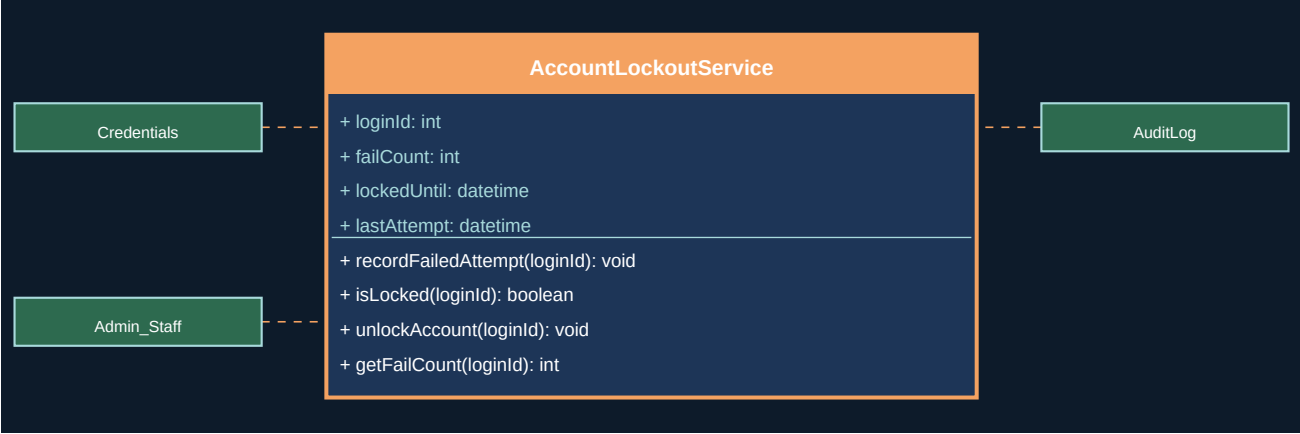
Figure 4.1 - UML Class Diagram
