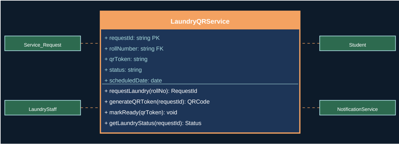
Figure 28.1 - UML Class Diagram
