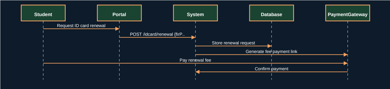
Figure 10.2 - UML Sequence Diagram
