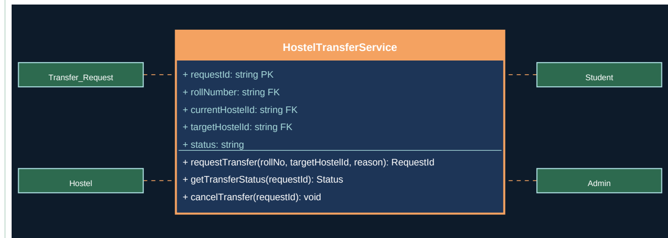
Figure 24.1 - UML Class Diagram
