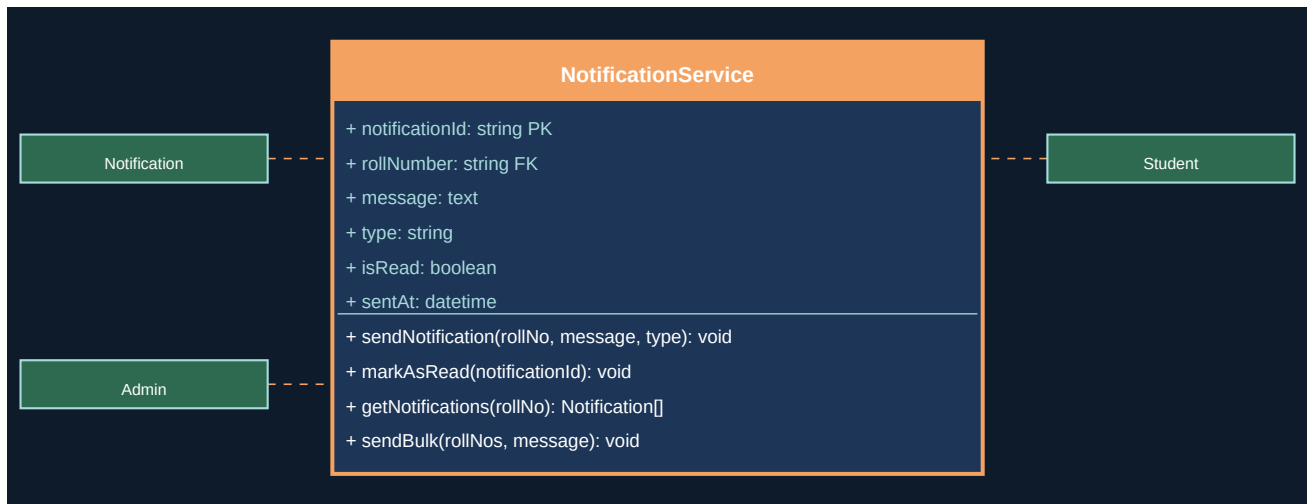
Figure 16.1 - UML Class Diagram
