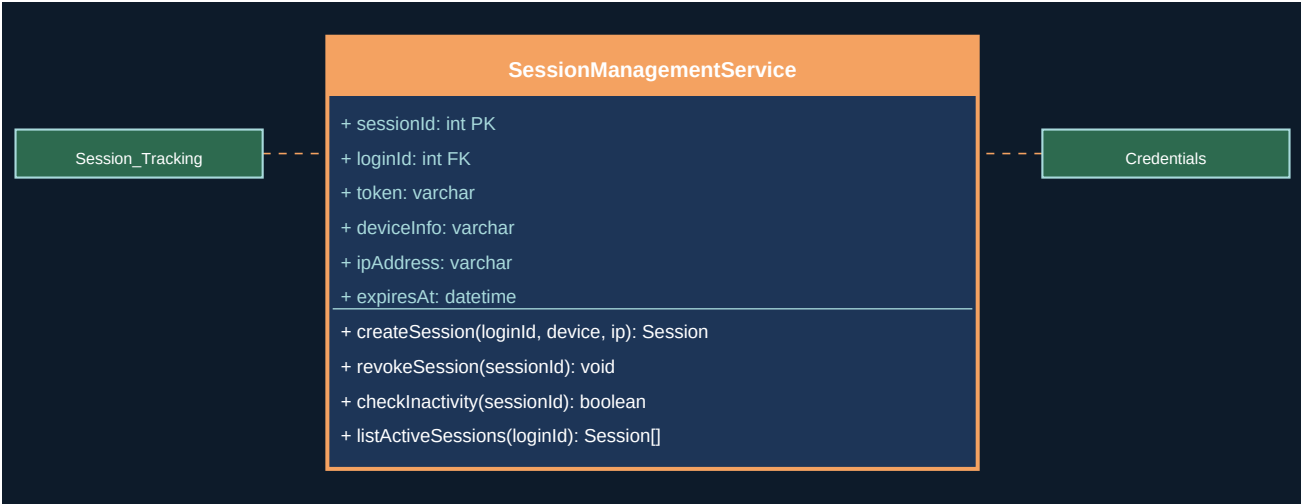
Figure 3.1 - UML Class Diagram
