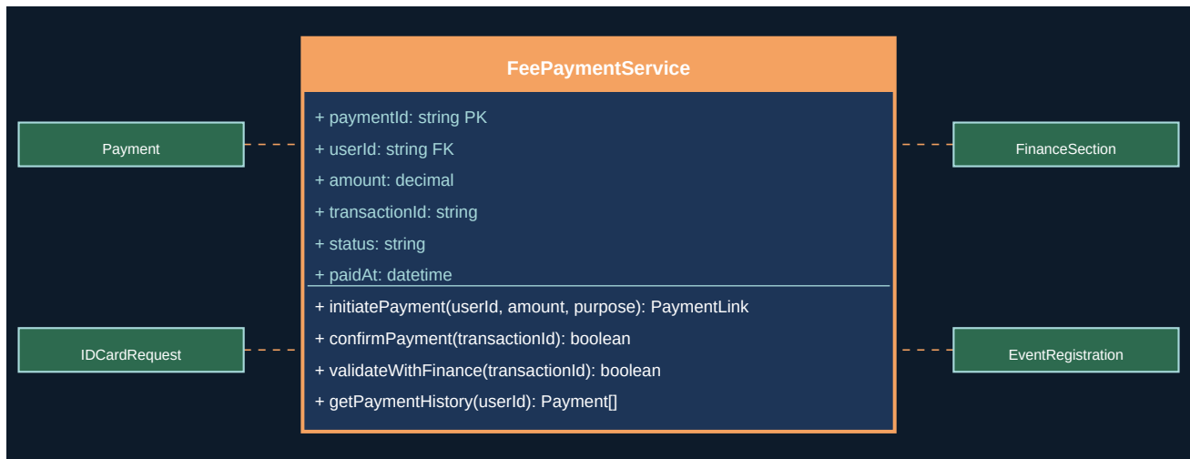
Figure 11.1 - UML Class Diagram
