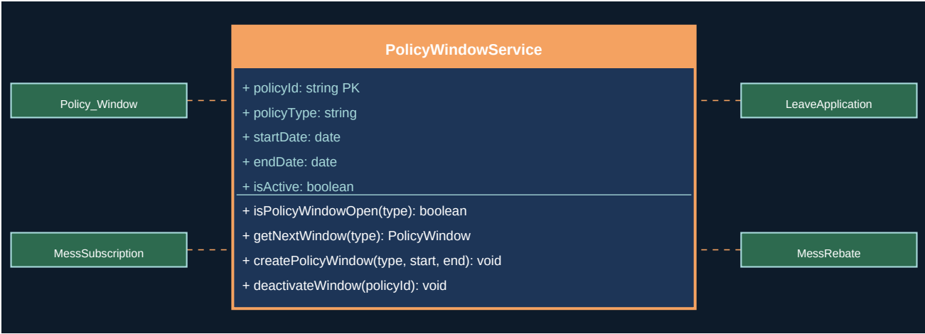
Figure 29.1 - UML Class Diagram
