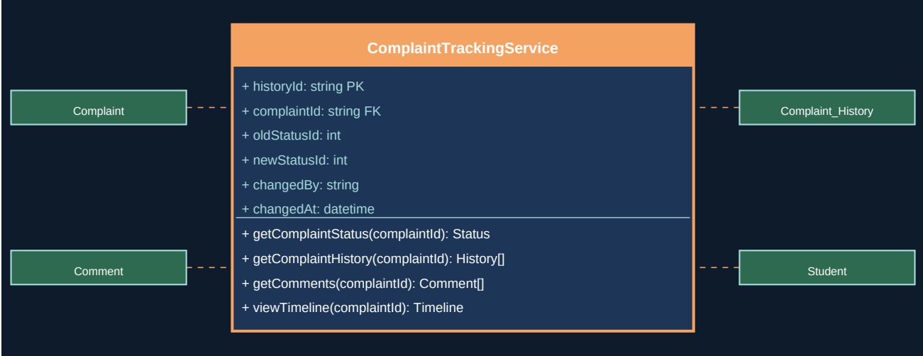
Figure 33.1 - UML Class Diagram
