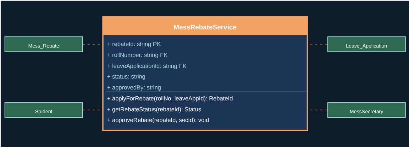
Figure 26.1 - UML Class Diagram
