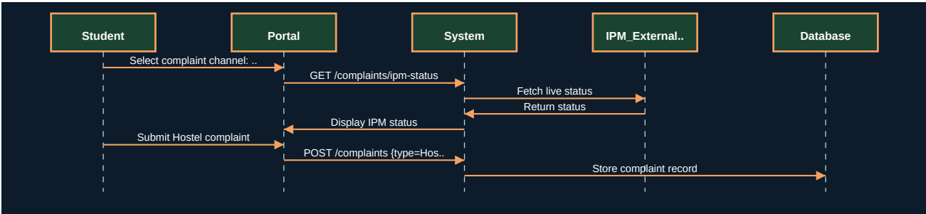
Figure 20.2 - UML Sequence Diagram
