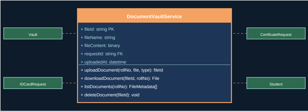
Figure 15.1 - UML Class Diagram
