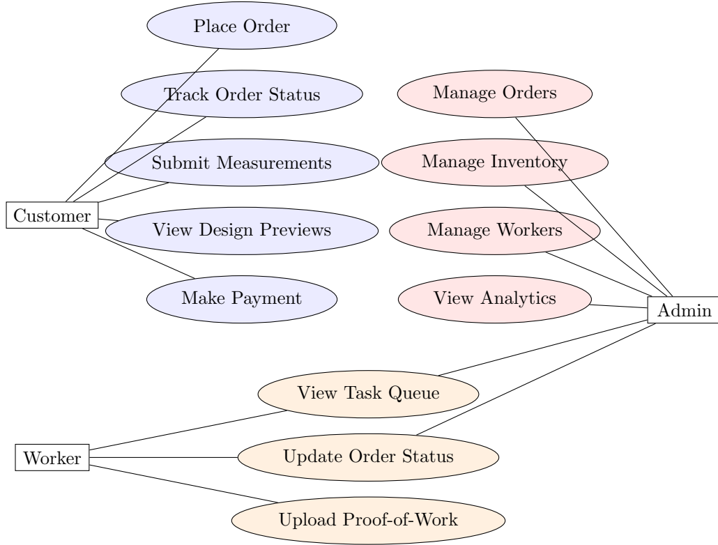
Figure 2: Use Case Diagram for StitchPerfect
