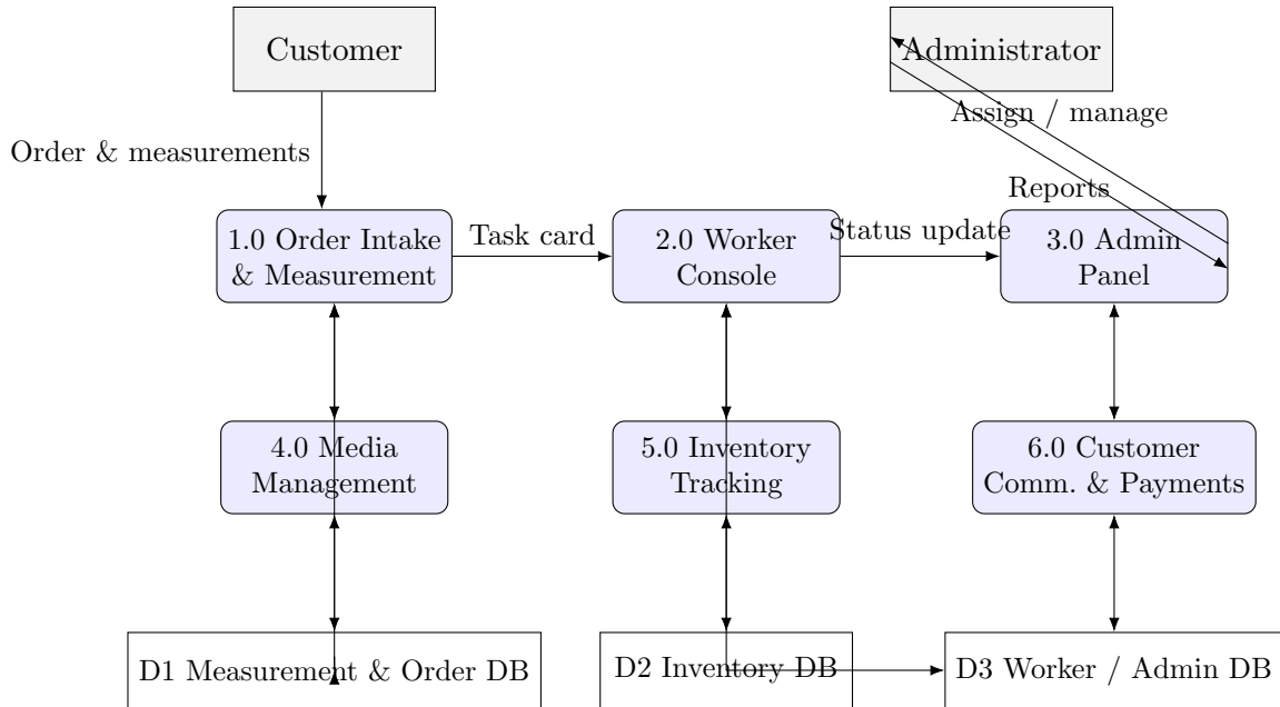
Figure 3: Level-1 Data Flow Diagram for StitchPerfect
