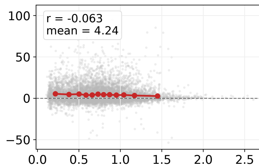
vs. FlowMatch
