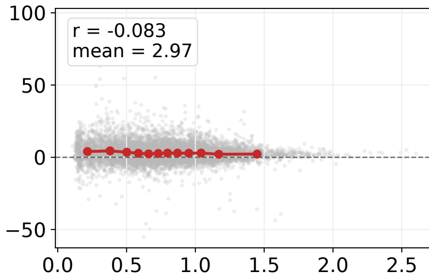
vs. ResShift
