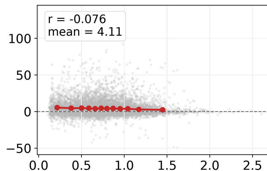
vs. FlowRefiner-ODE
