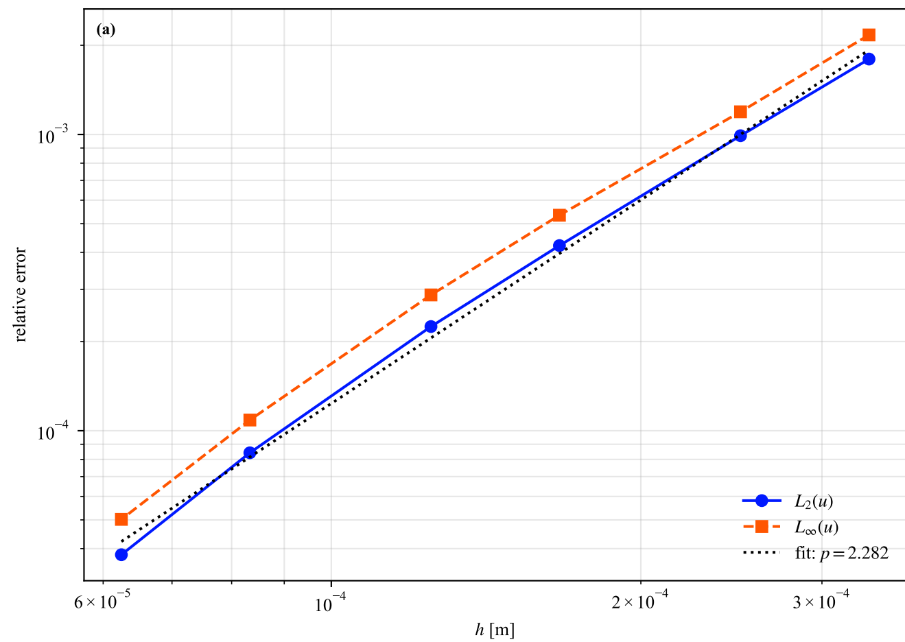
FVM error order and grid-independence study (reference: N=241)
