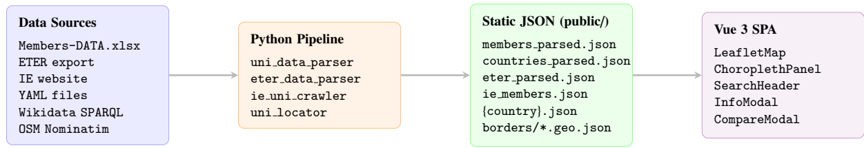
Figure 1: Diagram of data flow. Offline Python scripts transform raw data from Excel, YAML, and web sources into static JSON files. The Vue 3 SPA fetches these files at runtime and renders them as interactive maps and charts.
