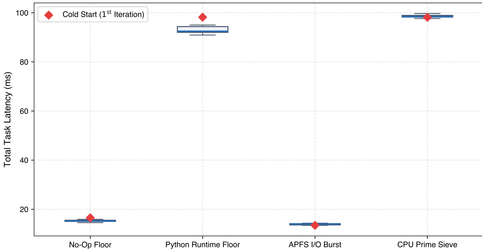
Figure 2: Empirical Latency Distribution & Cold Start Overhead (Seatbelt)
