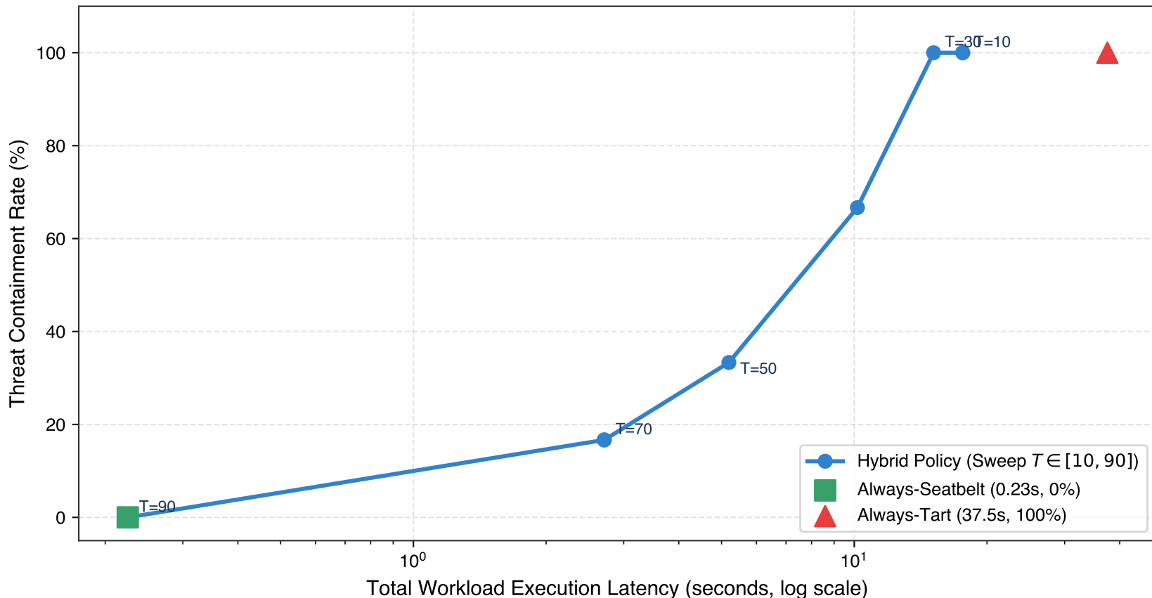
Figure 4: Latency vs. Containment Tradeoff Frontier (Hybrid Policy Sensitivity)
