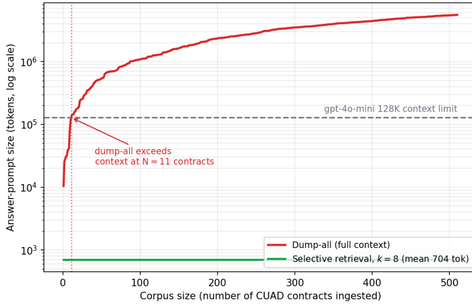
Figure 4.6: Answer-prompt size versus corpus size on CUAD (log scale). The full-context dump-all prompt grows linearly and exceeds the answerer’s 128K-token context at N \approx 11 contracts (reaching \approx 43 \times the limit at N=510 ); selective retrieval stays flat at \sim 704 tokens. Beyond N \approx 11 , dump-all must truncate and lose evidence; selective memory is unaffected.
